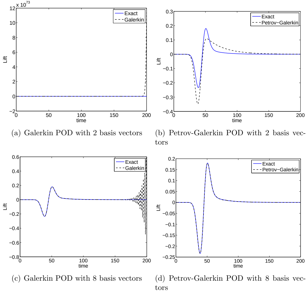
Figure 6-1: Comparison between the conventional Galerkin projection and the Petrov-Galerkin projection approaches. Solid lines are the full (exact) solution and dashed lines are reduced model results.
