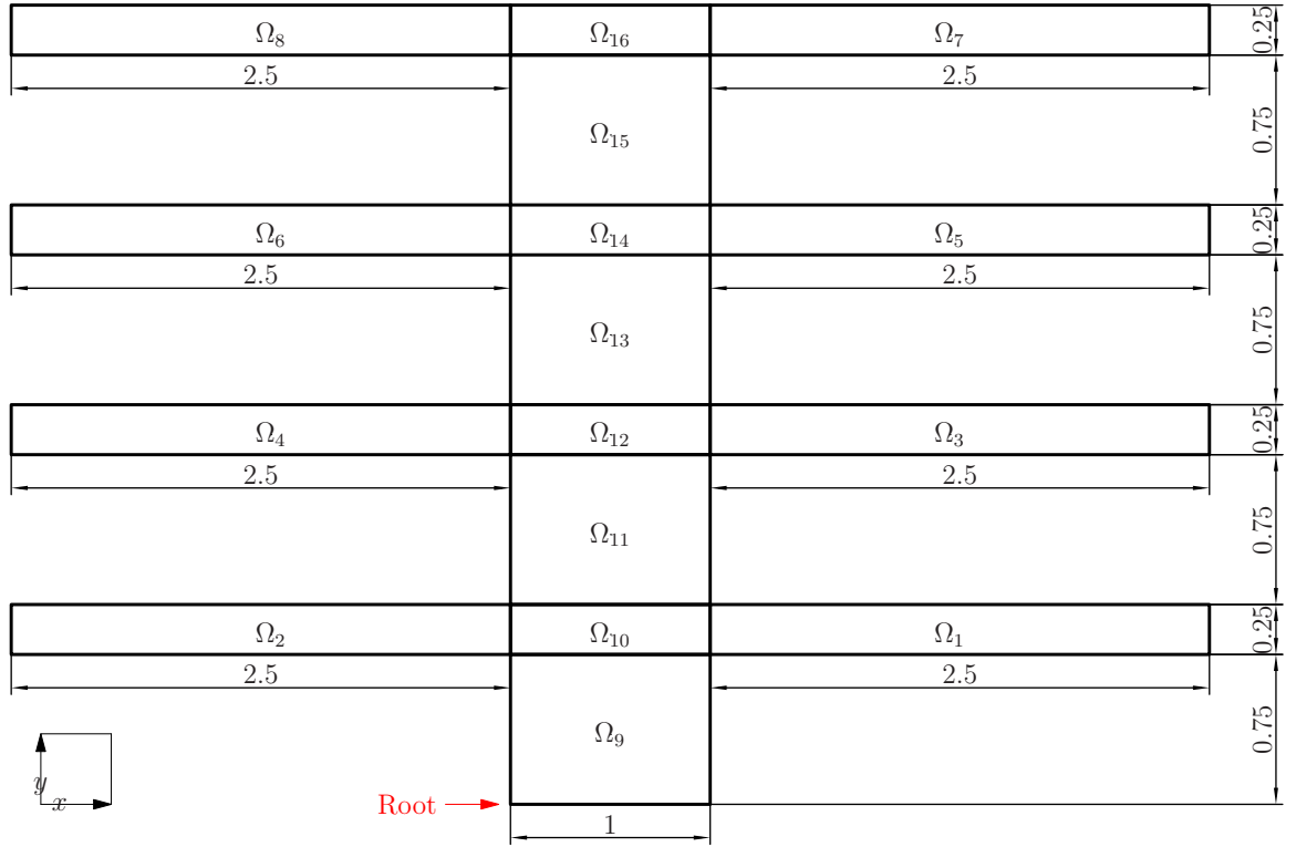
Figure 4-2: The thermal fin geometry in the computational domain.
