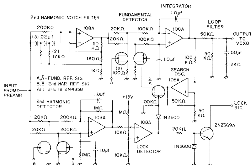
Figure 11 - Basic servo amplifier circuit
