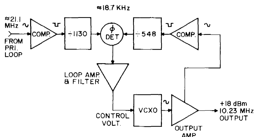
Figure 13 — Synthesizer block diagram
