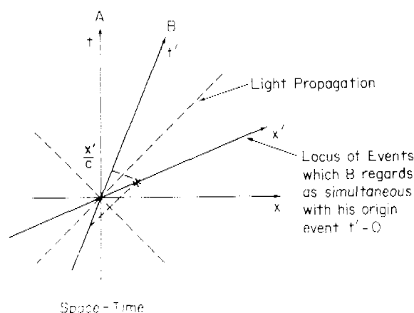
Figure 7 Minkowski's Absolute Space-Time (1907)
