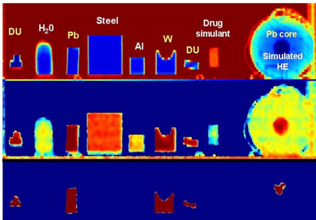
Figure 8. Dual-Energy Radiography
