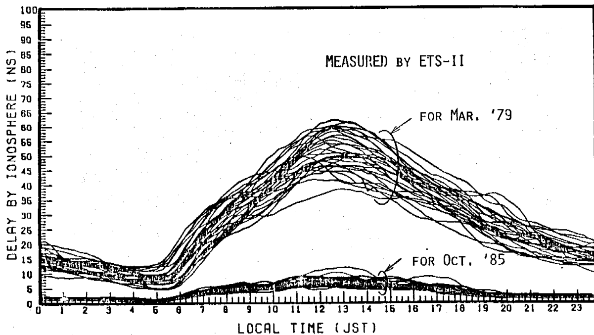
Figure 4. Example of the ionospheric effects on GPS L1 signal (calculated by the daily TEC measured) during solar maximum (1979) and near solar minimum (1985).
