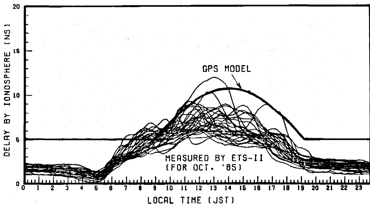
Figure 5. Comparison between the actual ionospheric effect on GPS L1 signal and ionospheric compensation model transmitted from GPS satellites.
