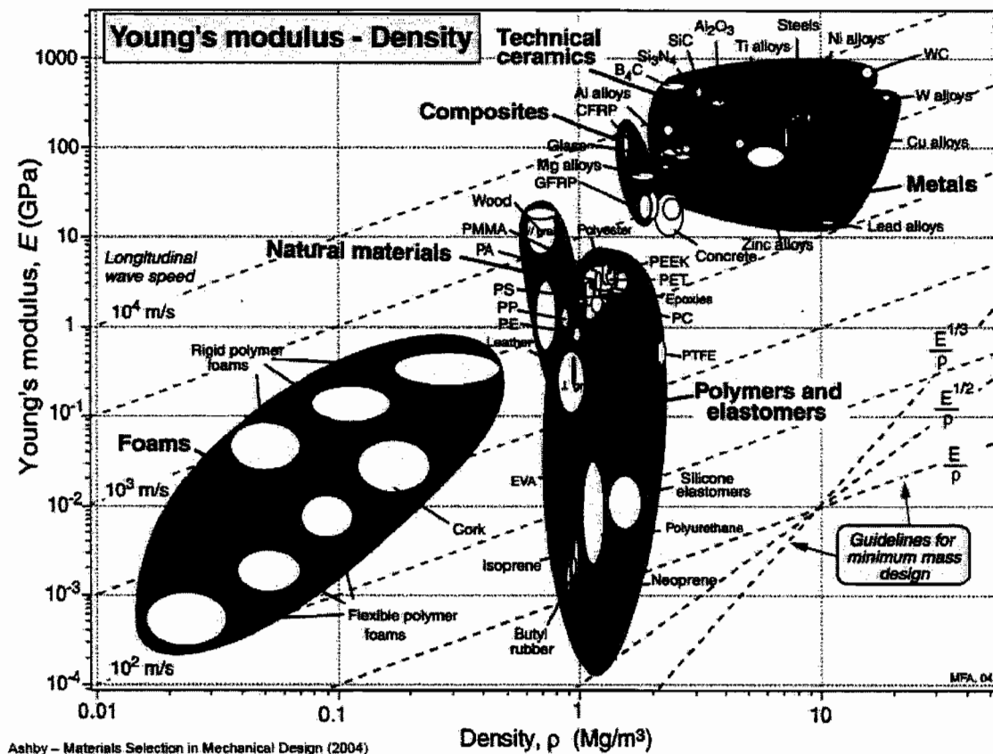
Figure 2.7: Ashby's MSC for Young's Modulus, E , against Density, \rho [13]
