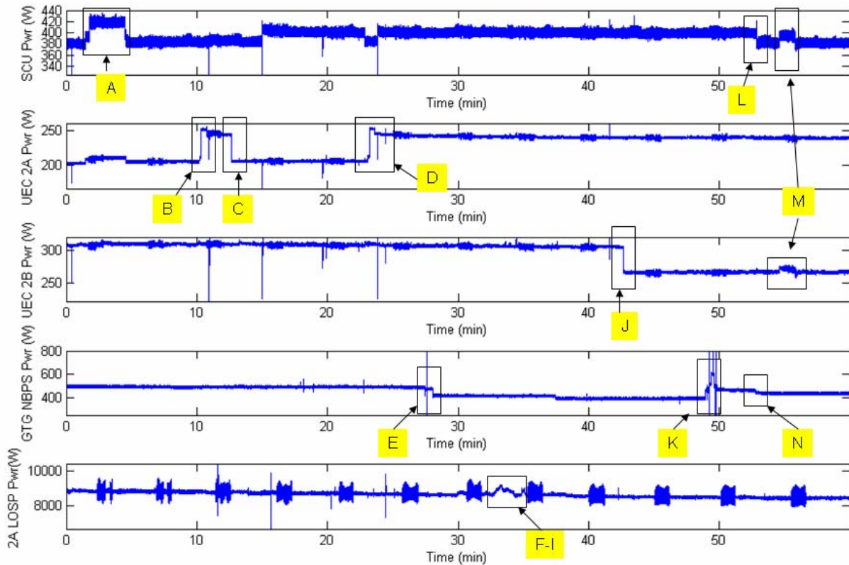
Figure 5-20: Time Aligned Plot showing power traces of SCU, UEC 2A, UEC 2B, GTG NBPS, & 2A LOSP captured on 16 April 2007 0900-1000
