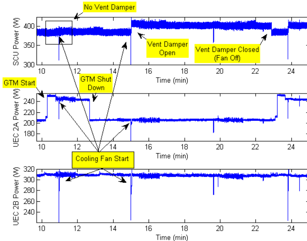
Figure 5-19: Vent Damper Failure Sequence
