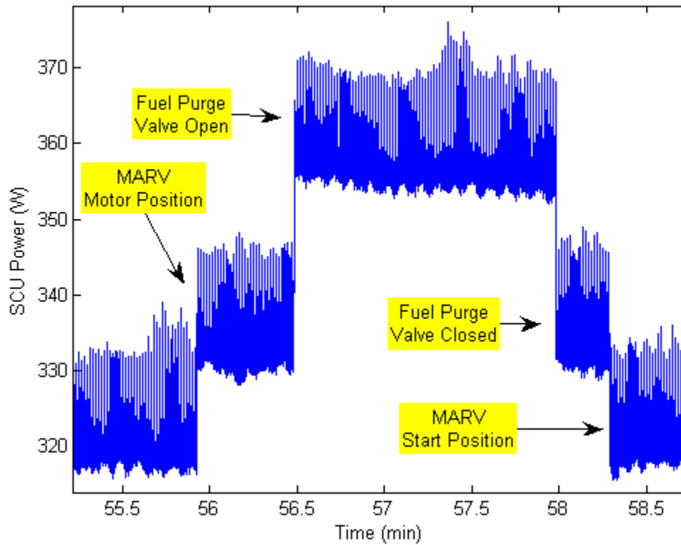
Figure 4-10: Power drawn by the SCU during a GTM motor and fuel purge
