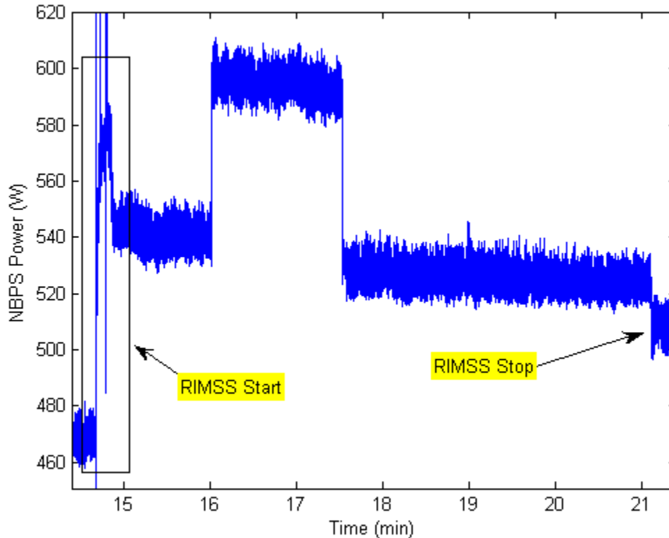
Figure 4-17: Power drawn by the GTG NBPS during a GTG motor
