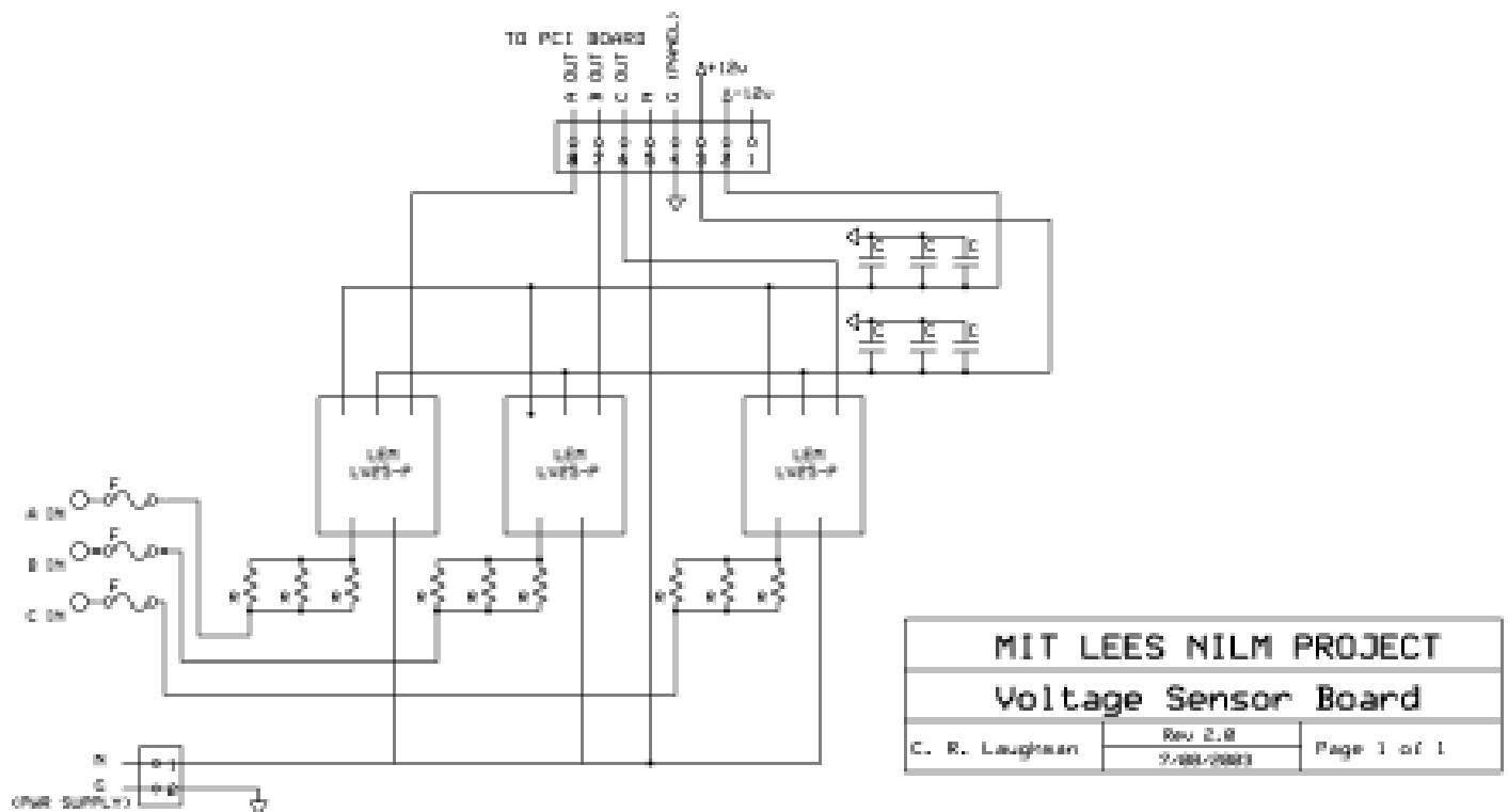
Figure 2-7: Voltage Board Circuit Diagram [45]
