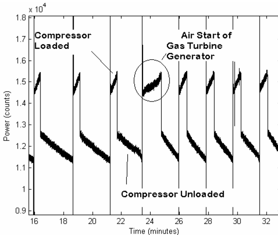
Figure 5-7: Plot of the real power drawn by the LPAC before, during, and after an air start of Nr 2 GTG. The units of real power are shown here to be counts, and they reflect the scale factors introduced by the NILM and were not converted to Watts [6].
