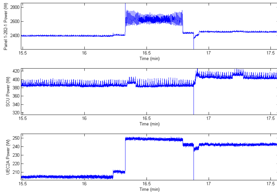
Figure 5-11: Power drawn during start of GTM 2A
