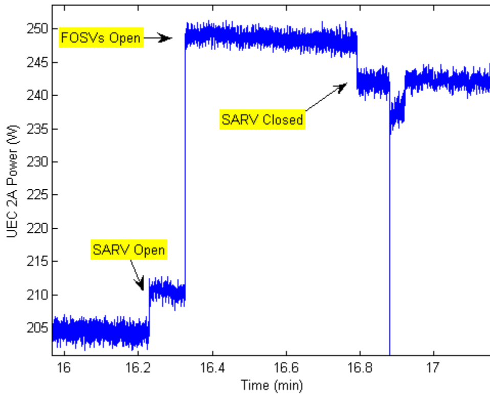
Figure 4-1: Power drawn by the UEC during a normal turbine start
