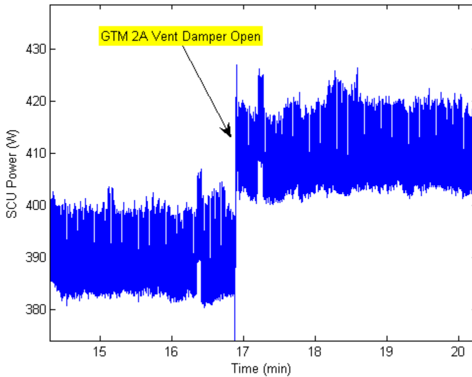
Figure 4-6: Power drawn by the SCU following a GTM start
