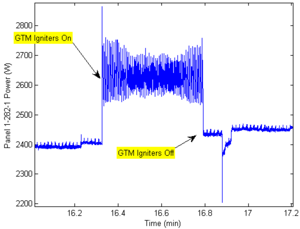
Figure 5-12: Close up of panel power drawn during the GTM 2A start shown in Figure 39
