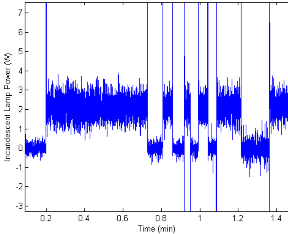
Figure 2-13: NILM power trace for an incandescent lamp taken during a NILM operational test.
