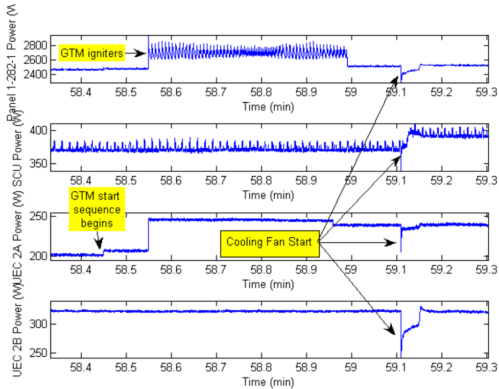
Figure 5-15: GTM Cooling Fan Starts
