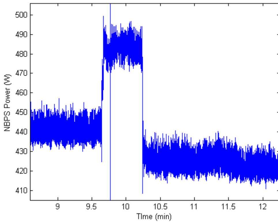
Figure 4-19: Power drawn by the GTG NBPS during a GTG Stop
