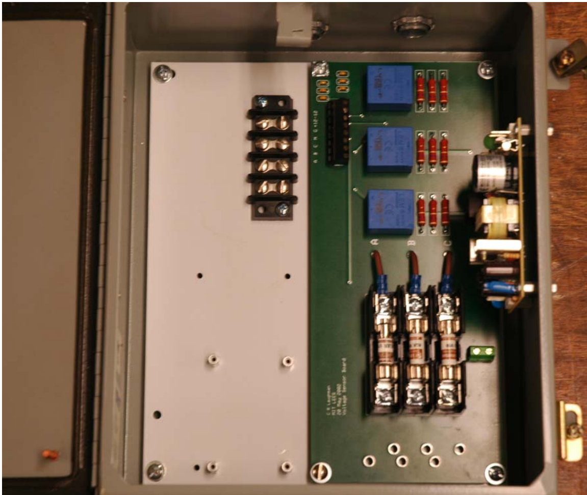
Figure 2-11: NILM Enclosure with Voltage Board and Power Supply Installed
