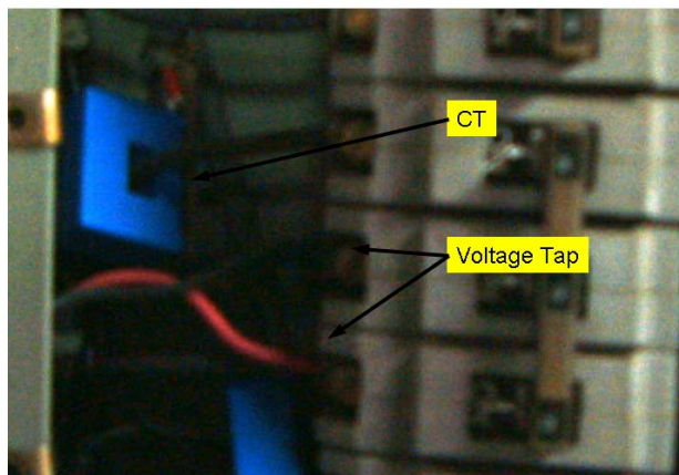
Figure 2-14: NILM CT and Voltage Tap Connections
