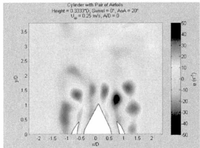
Figure 3-27: H 1/3, S 0, AoA 20 Picture
