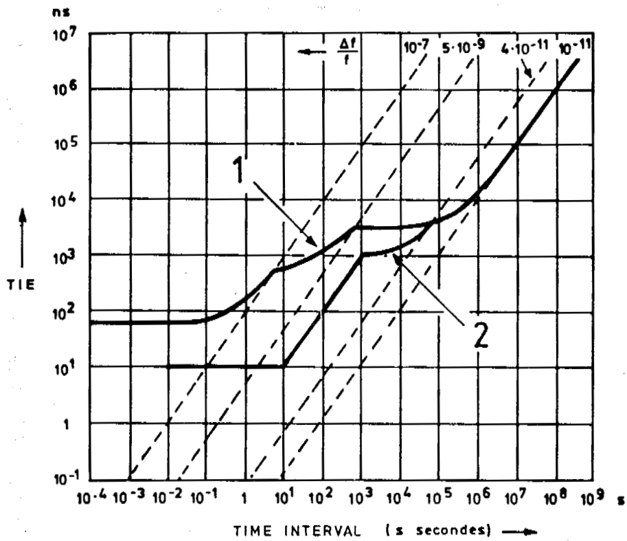
FIGURE 3 : TIE OUTPUT SIGNAL
