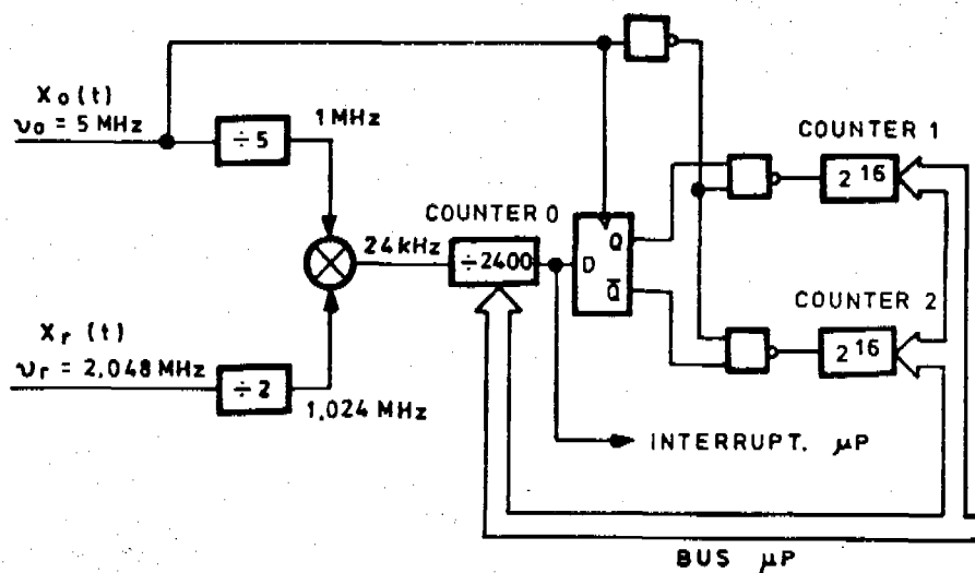
FIGURE 6 : PHASE COMPARATOR
