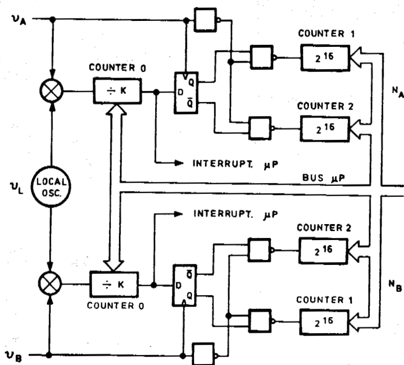
FIGURE 8 : MEASUREMENT OF TIE
