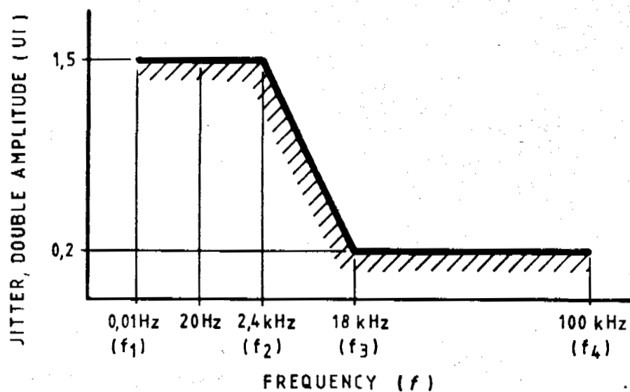
FIGURE 2 : JITTER INPUT SIGNAL
