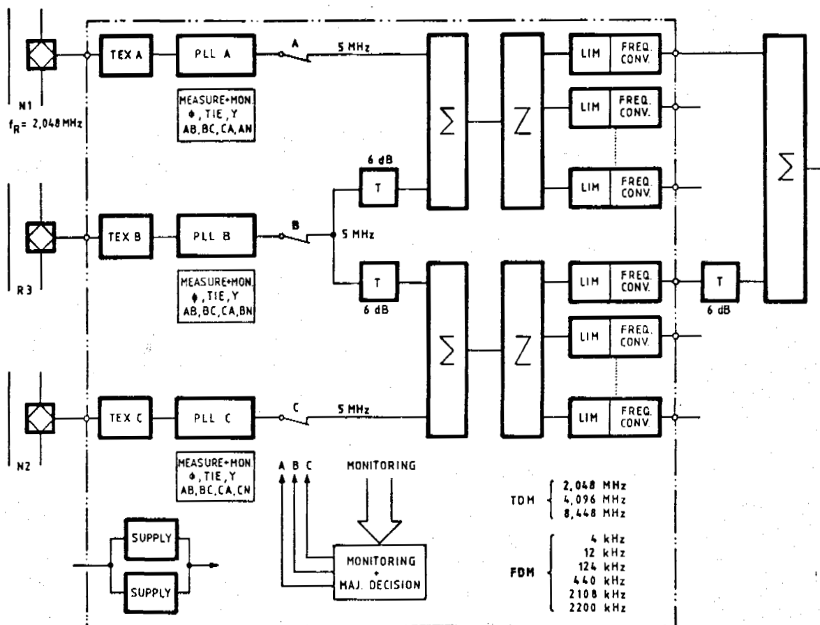
FIGURE 1 : GENERAL SCHEMATIC SECOND LEVEL CENTER
