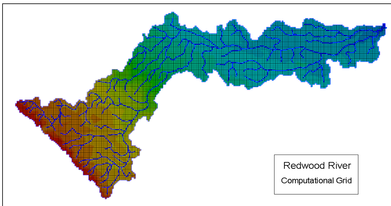
Figure 1. Representation of watershed, computational grid, and stream network in GSSHA.
