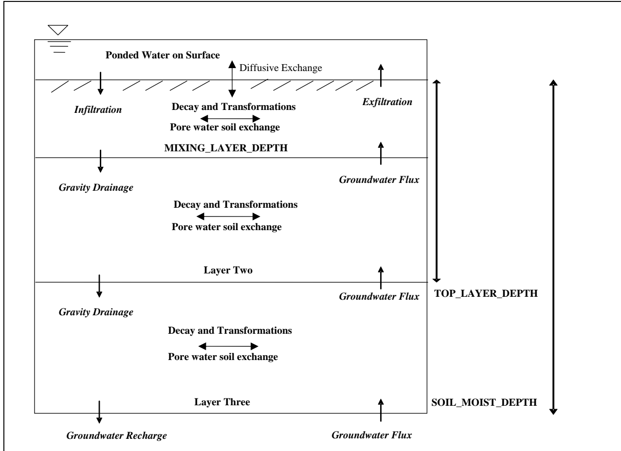
Figure 2. Soil column transport model.
