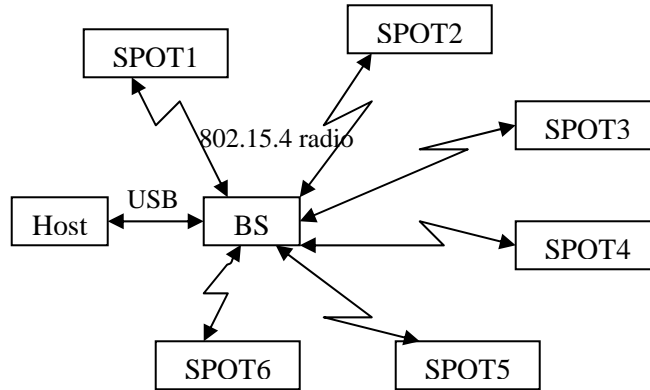
Figure 18. Star Topology
