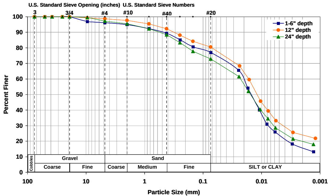
Figure 7-5. Summary of soil classification for the Cincinnati soil at each depth 0.6-m (2-ft) soil pits.
