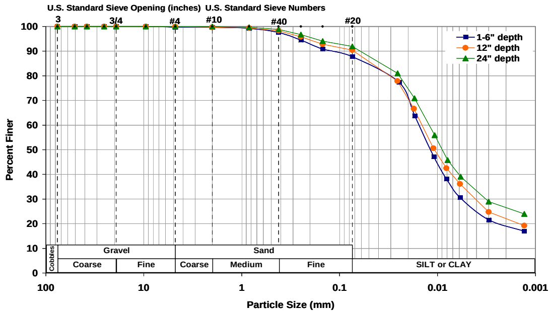
Figure 7-4. Summary of soil classification for the Cobbsfork soil at each depth 0.6-m (2-ft) soil pits.
