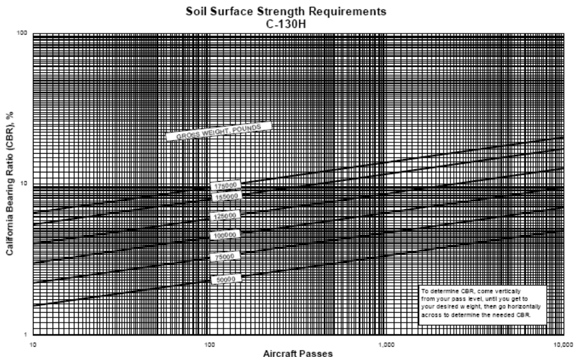
Figure 3-10. Chart to determine either allowable aircraft gross weight or allowable pass level for C-130 aircraft (from Air Force 2002).
