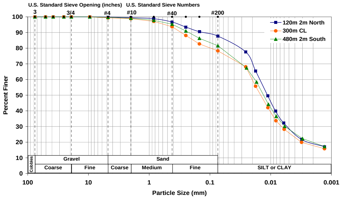
Figure B-3. Gradation analysis for 600-mm (24-in.) soil samples.
