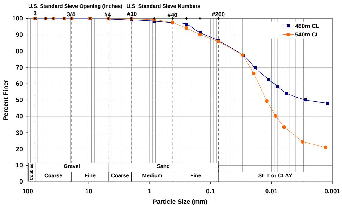
Figure B-4. Gradation analysis for 305- to 660-mm (12- to 26-in.) soil samples.
