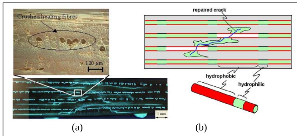
Figure 1. (a) A conventional vascular self-healing polymer (1) and (b) a concept for regulated self-pressurization through patterned surface properties.
