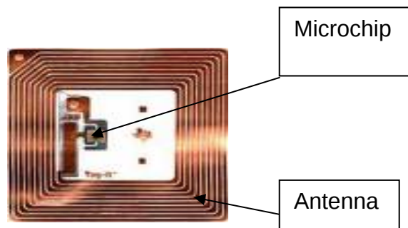
Figure 5. RFID tag
