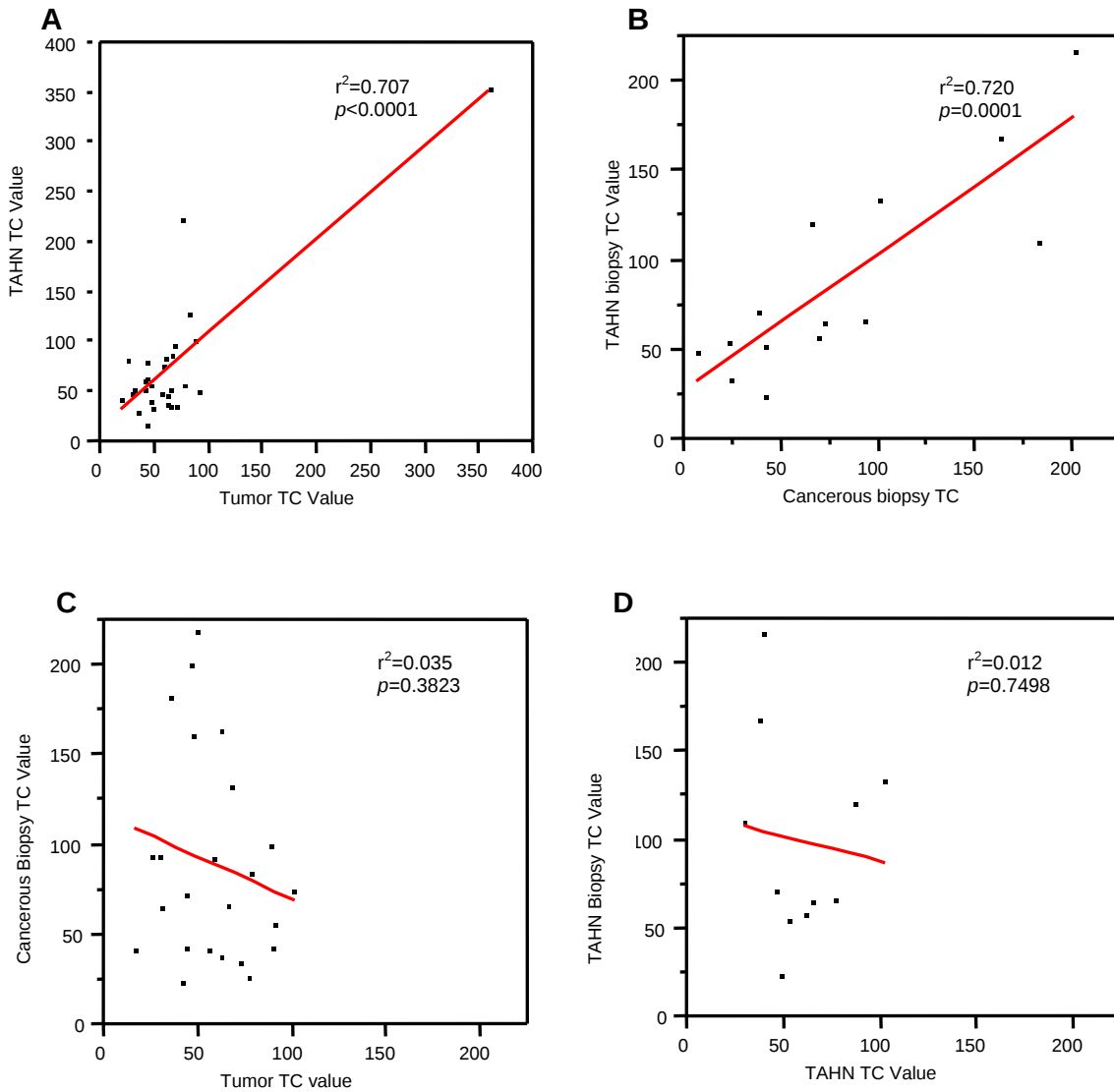
Figure 7. Correlation of samples by tissue source. Paired samples by prostatectomy or biopsy, and compared by relative tissue type. Panel A shows the TC relationship between TAHN and Tumor tissues. Panel shows the TC relationship between TAHN and Cancerous Biopsy tissues. Panel C shows the lack of TC correlation between Cancerous Biopsy and Tumor tissues. Panel D shows the lack of TC correlation between TAHN Biopsy and TAHN tissues.
