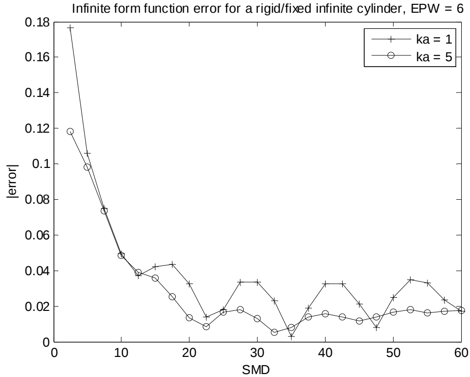
Figure 35 – Error in the infinite form function approximation of a rigid/fixed infinite cylinder at EPW = 6.
