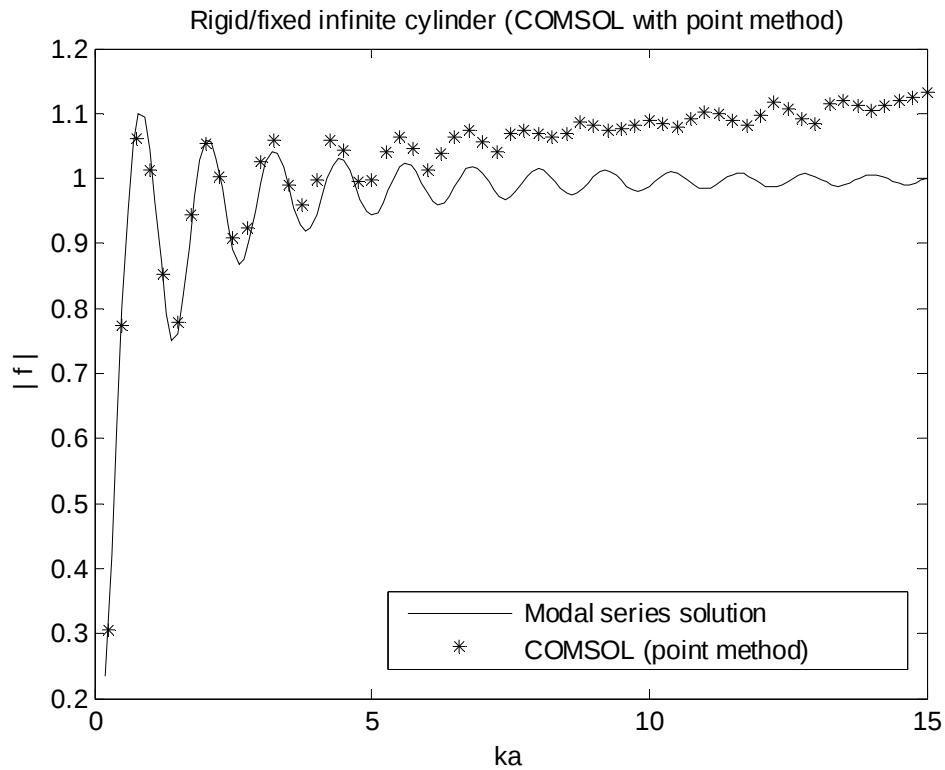
Figure 32 - Absolute value of infinite form function of a rigid/fixed infinite cylinder, using the modal series solution and COMSOL (point method). EPW = 6 and SMD = 50 .
