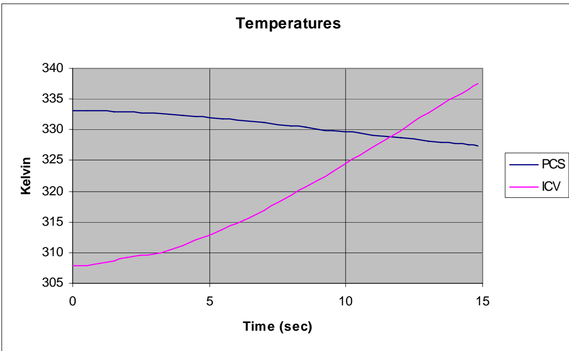
Figure A - 2 RELAP5 Temperature Data for PCS Discharge Simulation
