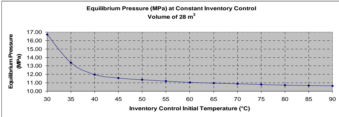
Figure 2.2.2 Effect on Equilibrium Pressure of Changing ICV Initial Temperature for emptying PCS
