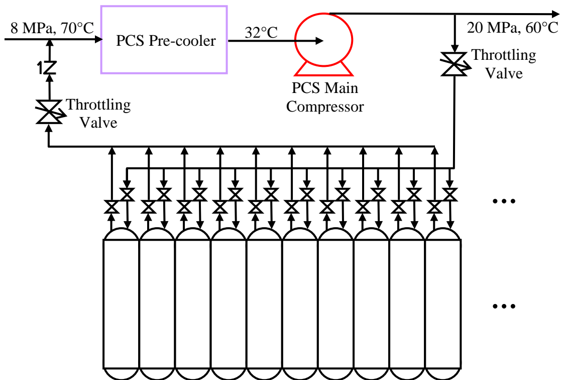
Figure 2.2.1 Proposed HPG storage system schematic for make-up and inventory control, without an additional compressor.
