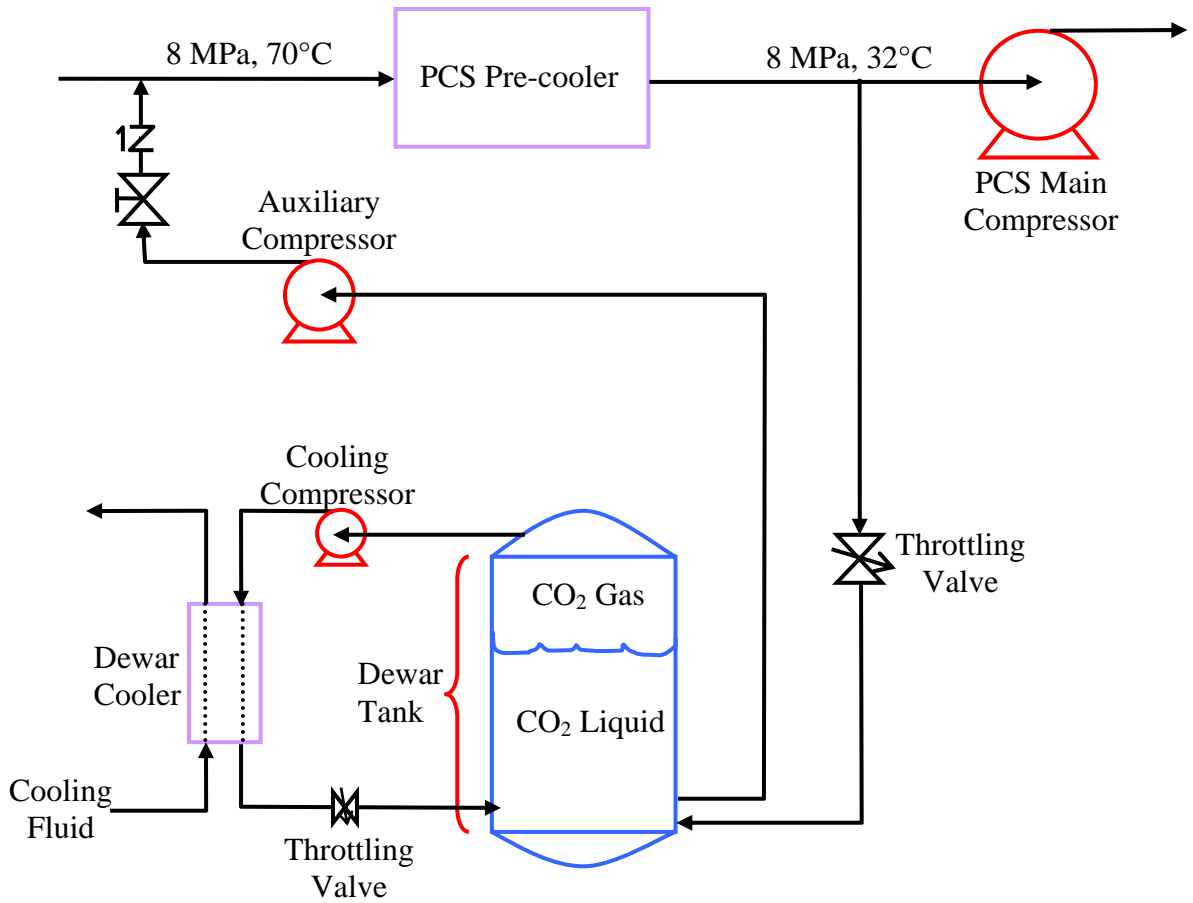
Figure 2.3.3 Proposed cryogenic system schematic for make-up, inventory control, and refrigeration
