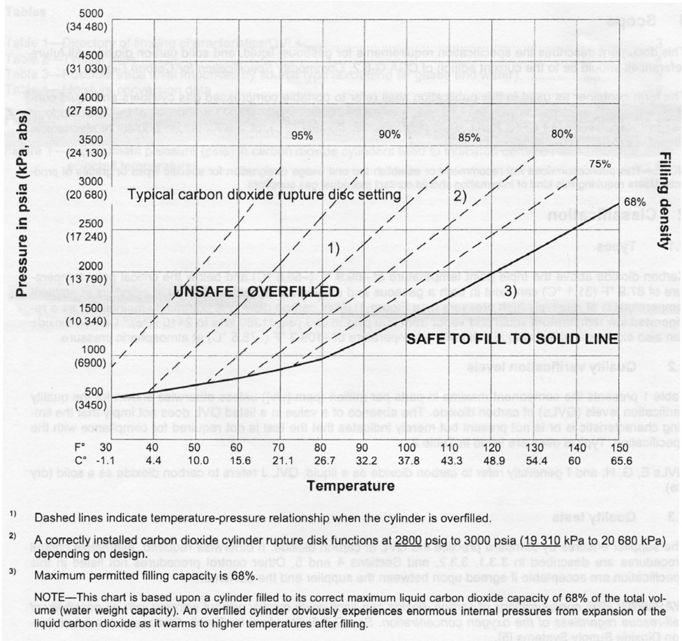
Figure 2.5.1 Temperature-Pressure relationship of CO 2 at various filling densities [CGA, 2004]*
