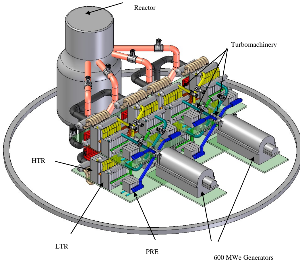
Figure 1.2.2 Isometric view of the 1200 MWe direct S-CO 2 PCS. Four parallel 300 MWe loops on two floors to achieve the total rated power [Gibbs, 2008].
