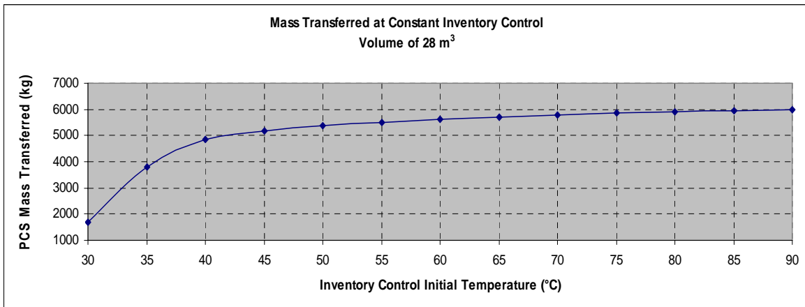
Figure 2.2.3 Effect on Mass Transferred of Changing ICV Initial Temperature for emptying PCS
