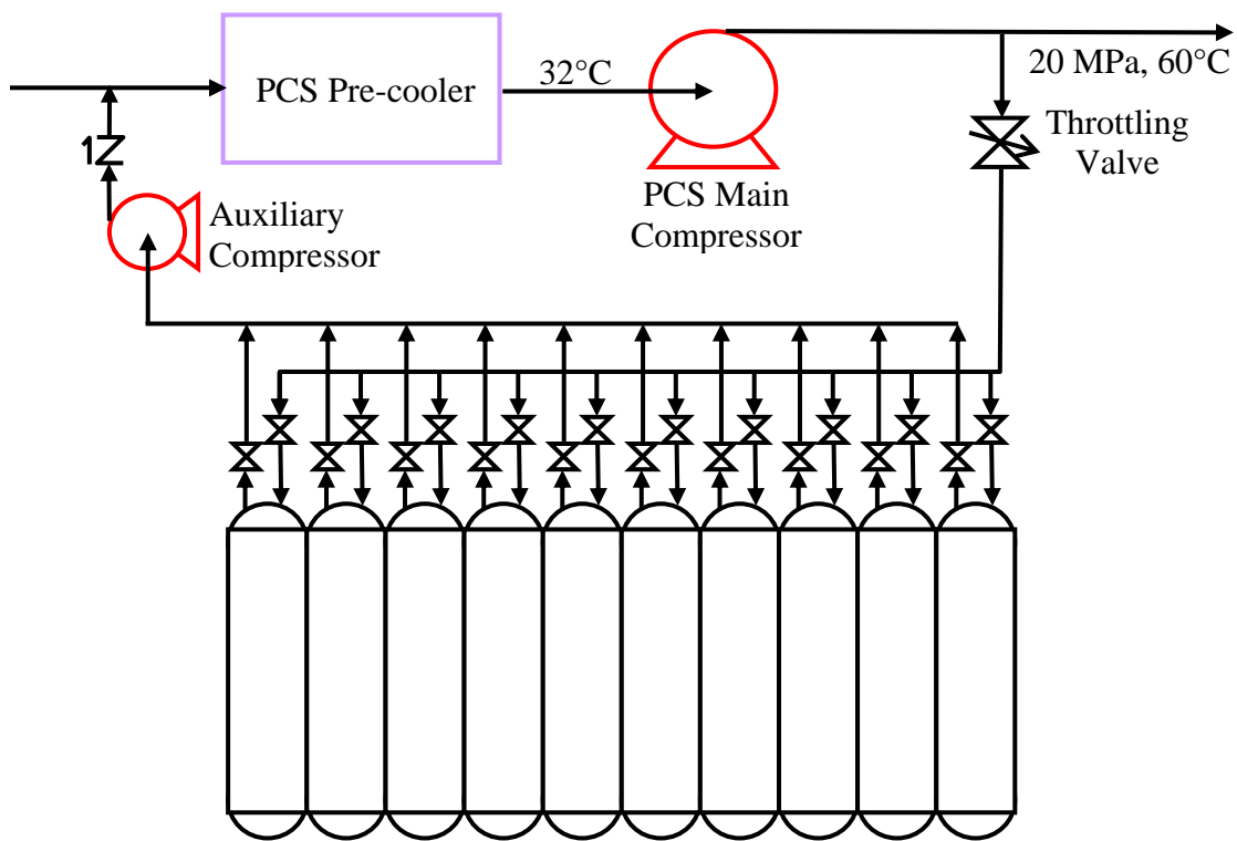
Figure 2.2.13 Proposed HPG storage system schematic for make-up and inventory control, with compression.
