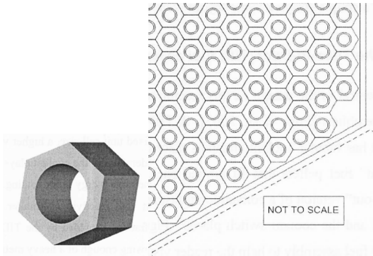
Figure D - 6 UO 2 fuel pellet (left) and quarter cross-section of the TID fuel assembly (right).
