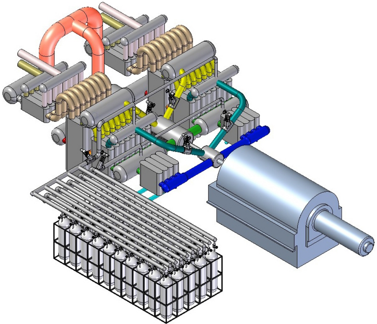
Figure C - 1 Isometric view of the 300 MWe Indirect Power Conversion System loop with HPG Storage (50 tanks, each 10 m 3 )
