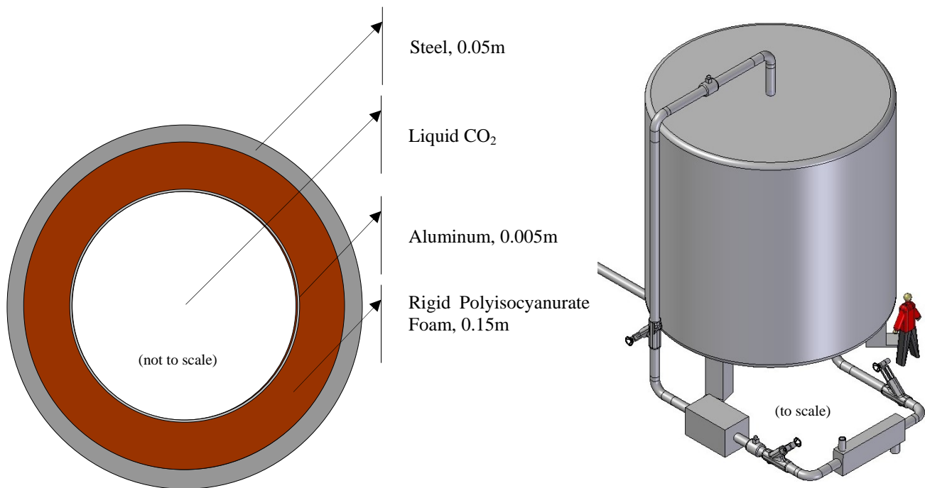
Figure 2.3.4 Cross section and an isometric view of cryogenic tank. Man is 6 ft tall.
