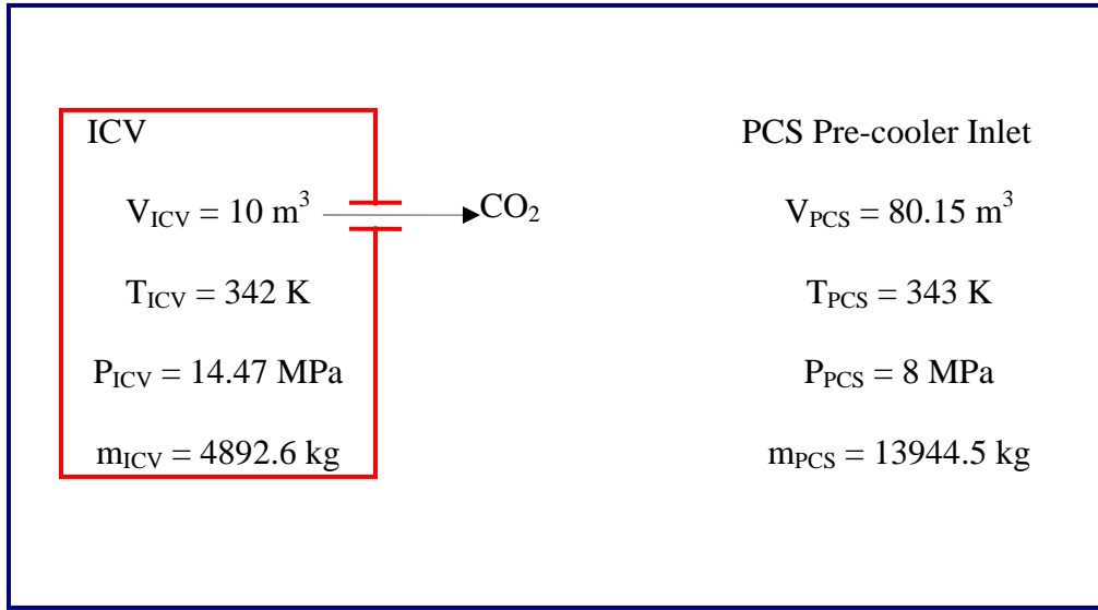
Figure 2.2.12 Simplified Model for discharging ICV into PCS Pre-cooler Inlet. V = Volume, T = Temperature, P = Pressure, and m = mass.
