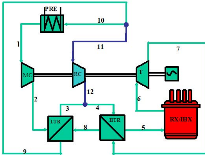
Figure 1.2.1 S-CO 2 Recompression Cycle Line Diagram [Dostal et al., 2004].
