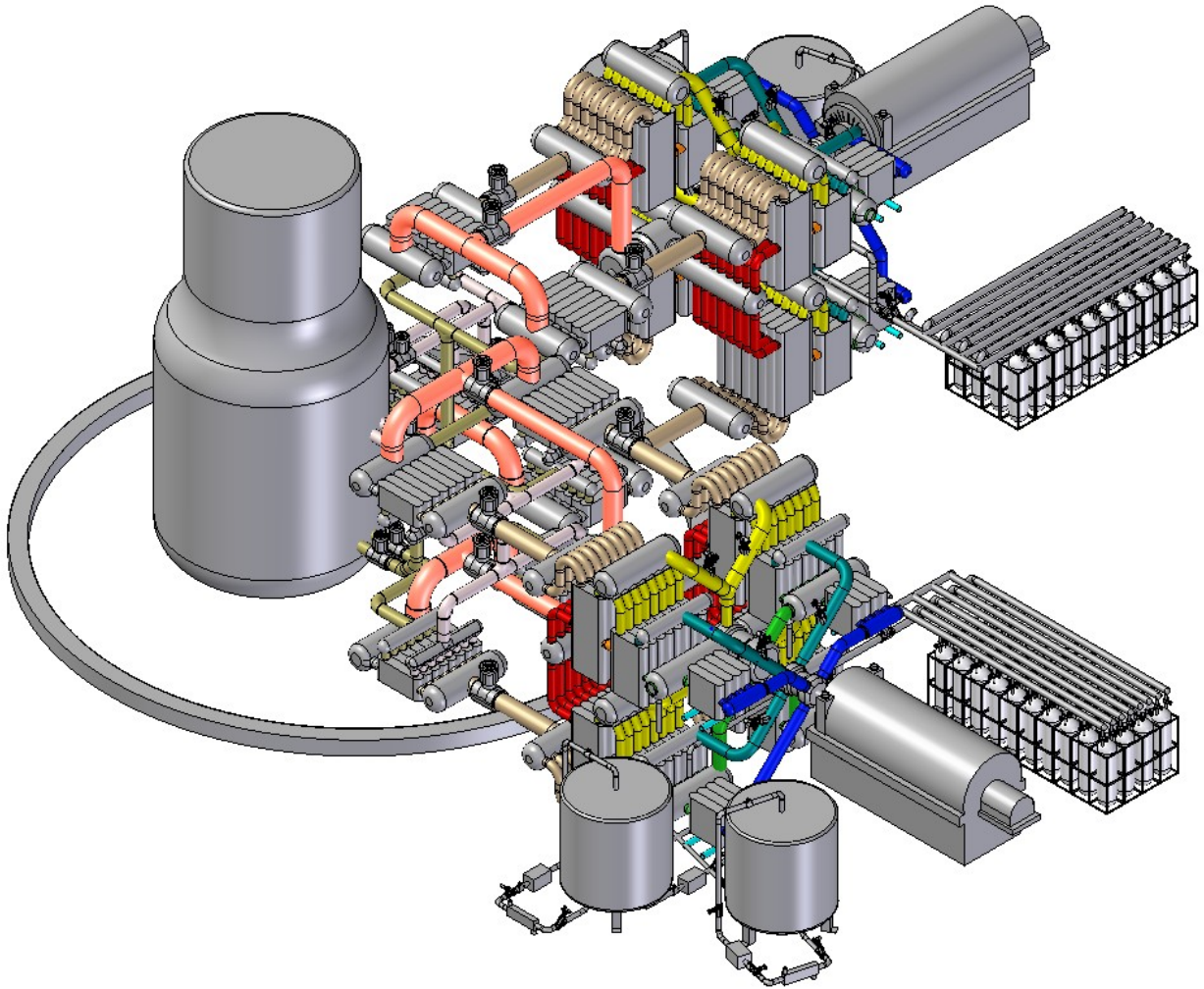
Figure C - 8 Isometric view of the 1200 MW e Indirect Power Conversion System with Cryogenic and HPG Storage
