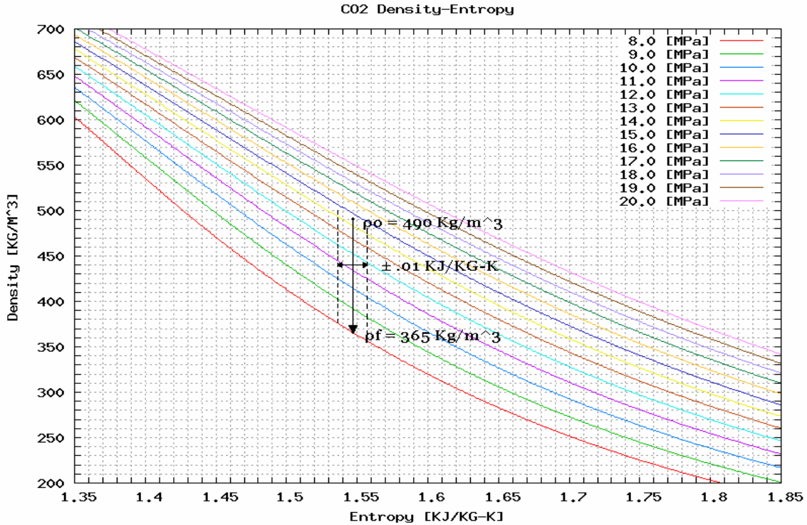
Figure 2.2.11 NIST \rho -s/P plot used in “pick-off” method for filling the PCS from Storage. Density vs. Entropy at varying Pressures for CO 2 . Using the initial and final conditions for the ICV, and the entropy found from figure 2.2.10, the change in density \Delta\rho = -125 \pm 5 kg/m 3 .
