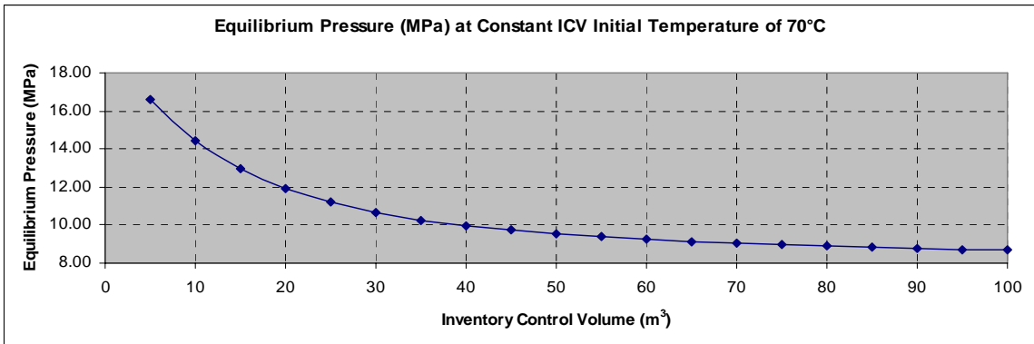
Figure 2.2.4 Effect on Equilibrium Pressure of Changing ICV Volume for emptying PCS
