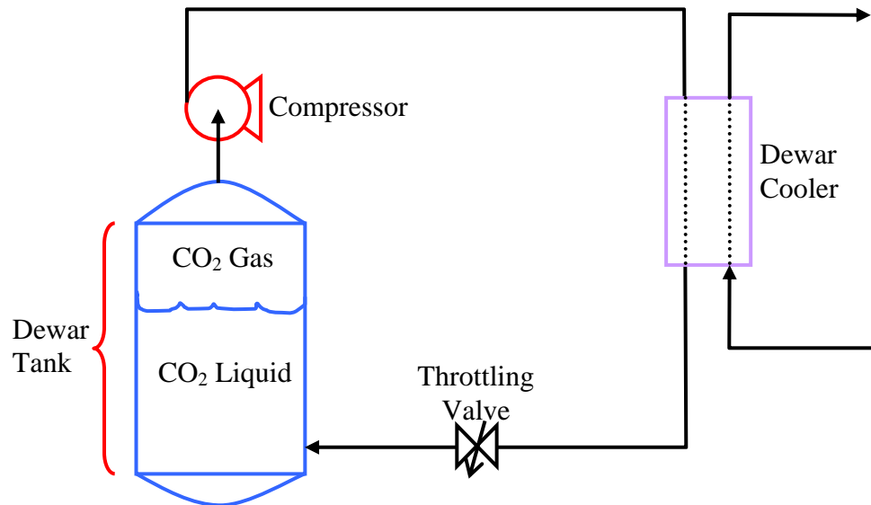
Figure 2.3.1 Dewar Tank with simple refrigeration loop
