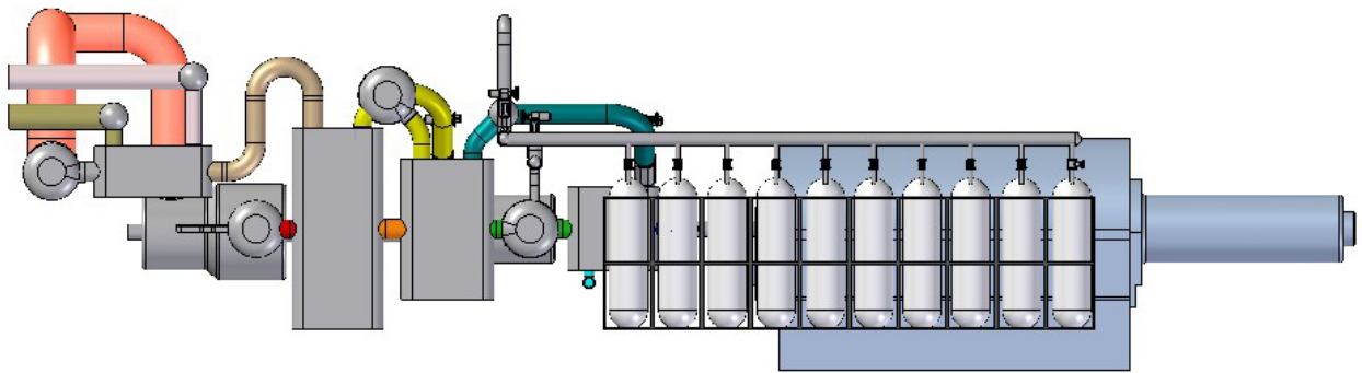
Figure C - 3 Side View of the 300 MW e Indirect PCS loop with HPG Storage
