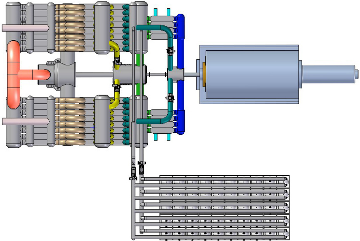
Figure C - 2 Top view of the 300 MW e Indirect PCS loop with HPG Storage
