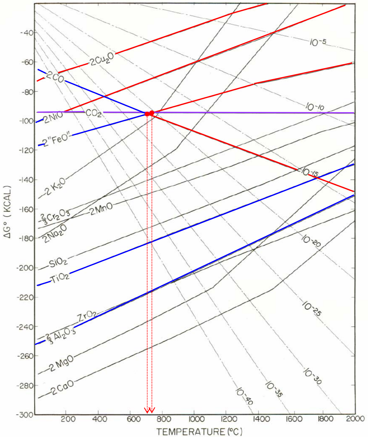
Figure D - 2 Simplified Ellingham Diagram. Solid curves showing standard free energies of formation of various oxides from the elements as a function of temperature, based mainly on data summarized by Coughlin and by Elliott and Gleiser. The curve for SiO 2 has been drawn on the basis of new data presented by Chipman. Light dash-dot curves are lines of equal oxygen pressures (atm) of the gas phase, as labeled on each curve.
