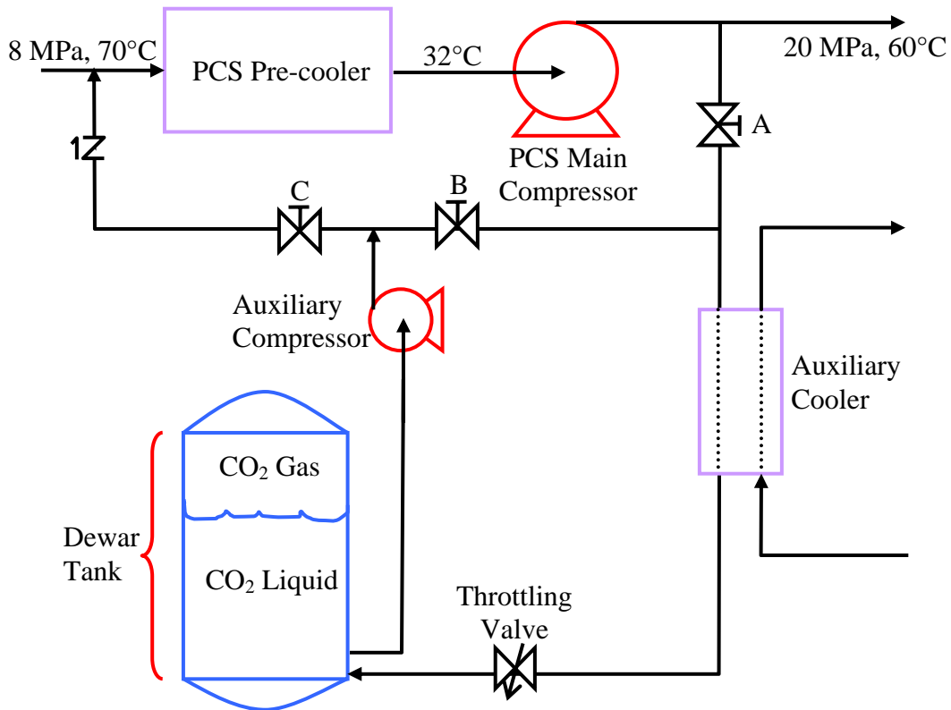
Figure 2.3.2 Possible way to combine make-up, inventory control, and refrigeration
