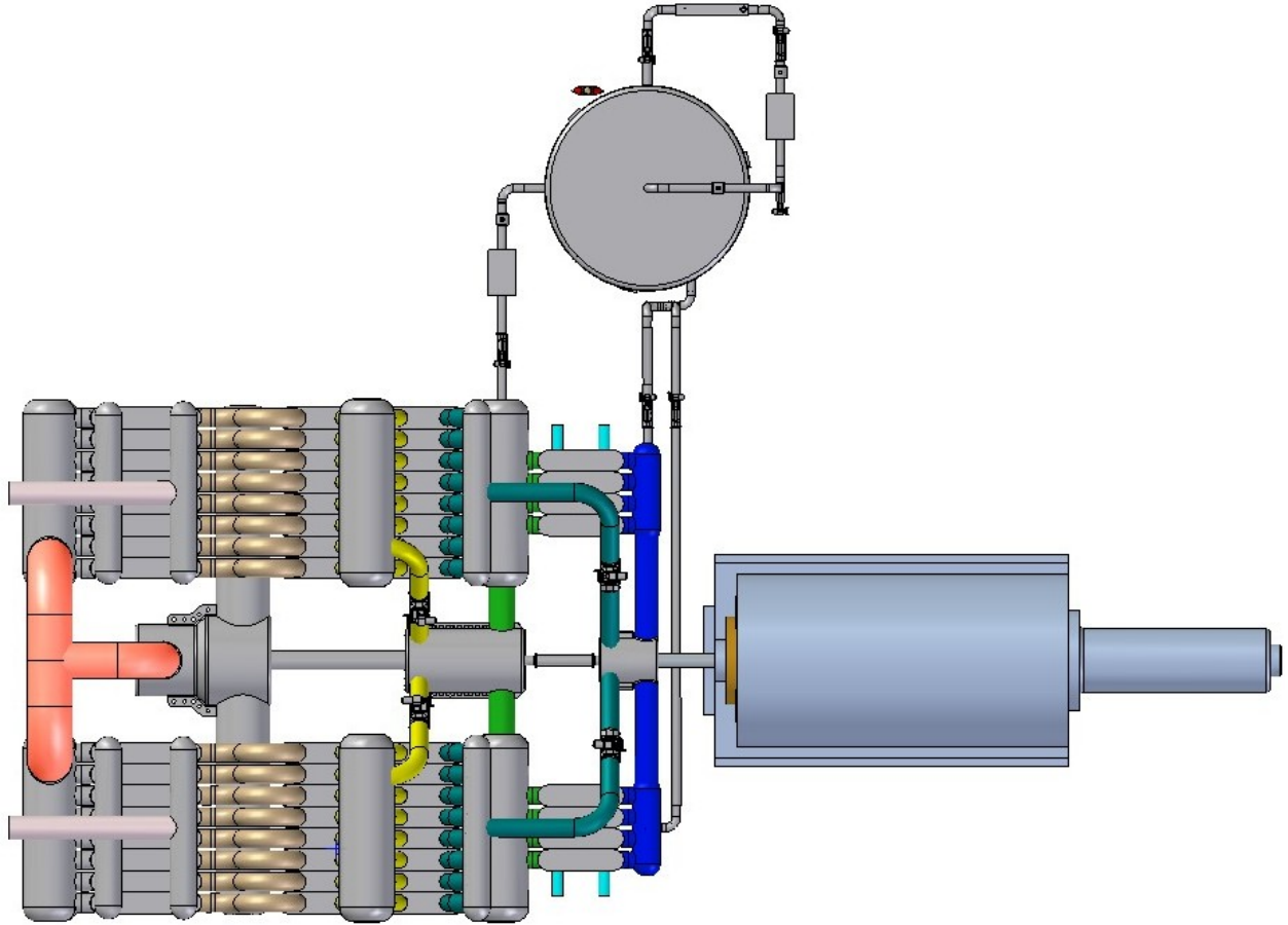
Figure C - 6 Top view of the 300 MW e Indirect PCS loop with Cryogenic Storage
