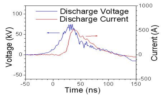
Fig. 5. Pseudospark pulse generator voltage and current applied to ignition reactor. For optimal operation current is approximately in phase with voltage for these applications.
