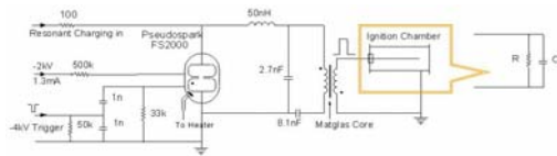
Fig. 4. Line-type pulser with pseudospark switch connected to ignition chamber for flame ignition studies.
