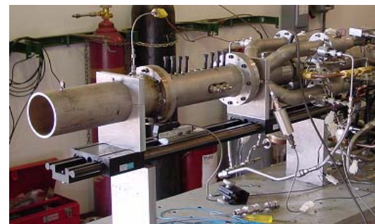
Fig. 6. Pulse detonation engine at the Naval Postgraduate School Rocket Propulsion Laboratory.
