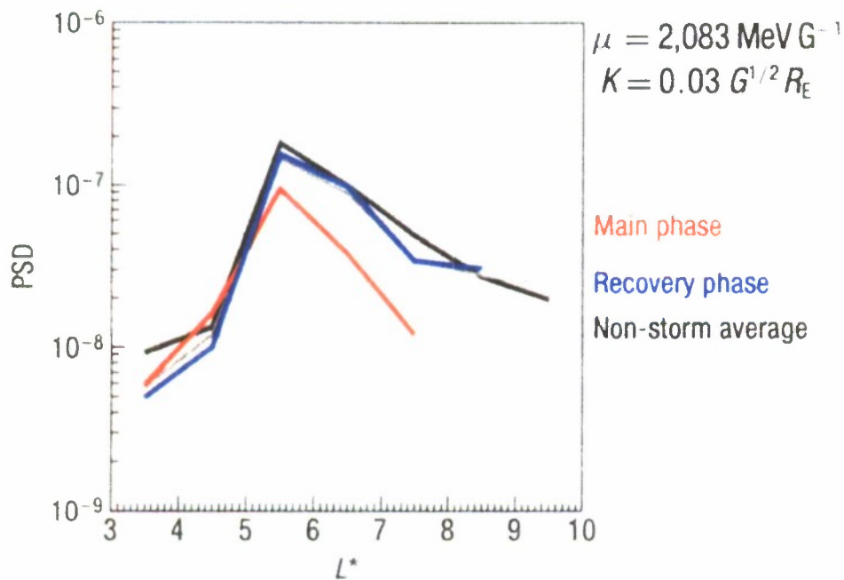
Figure 6. PSD radial profiles from Multisatellite observations during storm main and recovery phases plus comparisons to average PSD profiles. (after Chen et al. 2007).
