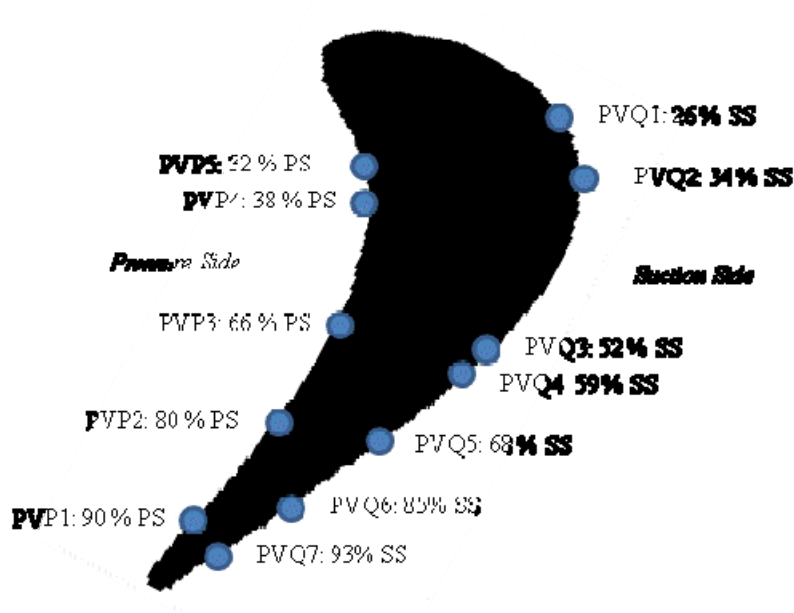
Figure 24: 60 % Span pressure transducers
