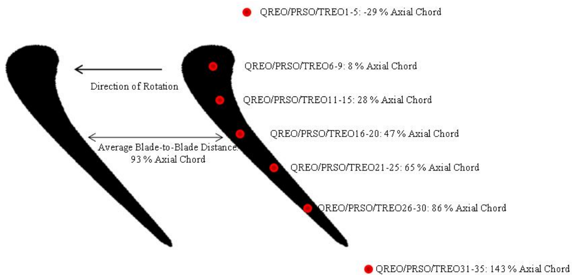
Figure 25: BOAS-mounted gauges
