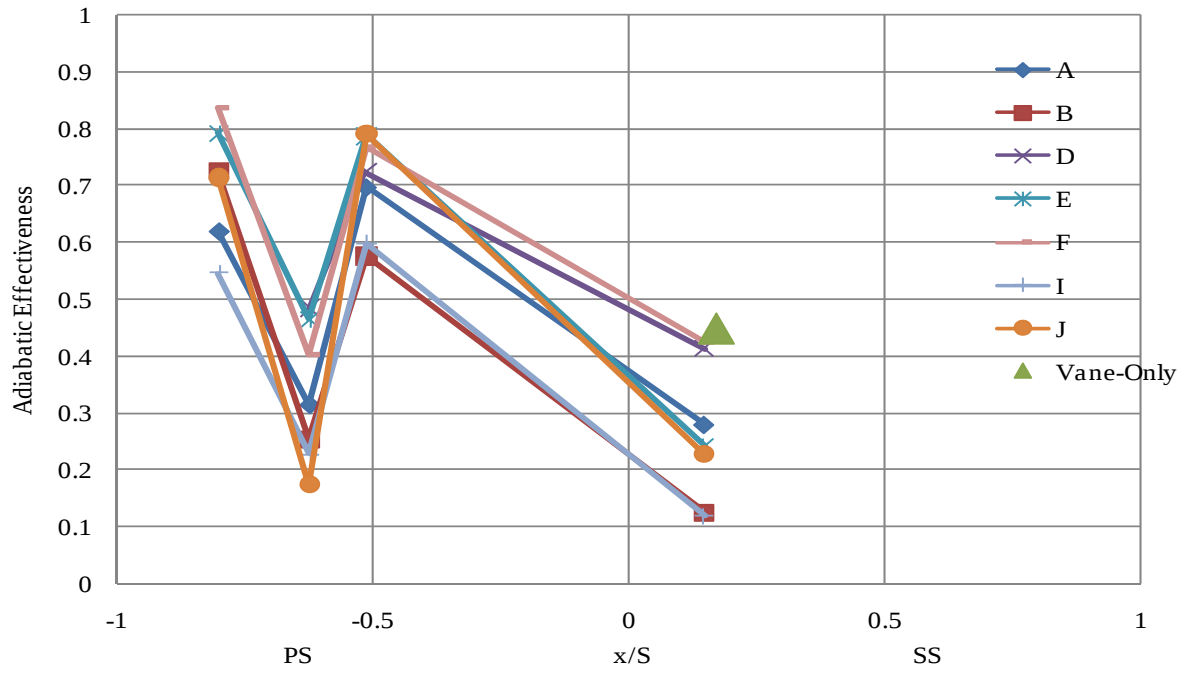
Figure 70: Adiabatic film-cooled effectiveness along vane surface, 60 % span
