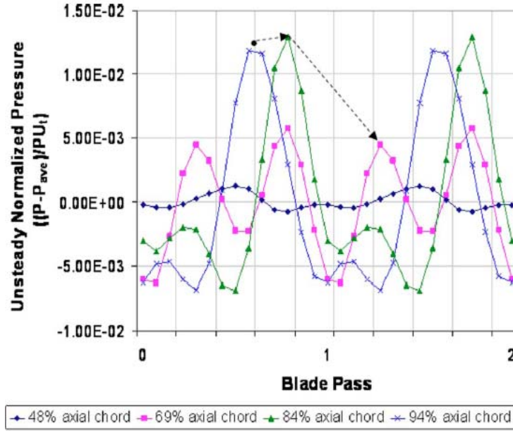
Figure 4: Unsteady, normalized pressure disturbances on vane suction surface (from Urbassik, 2003)
