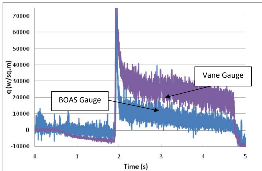
Figure 44: Heat flux histories—Run 1, 47 % x/C BOAS and 90 % SS vane, 60 % span
