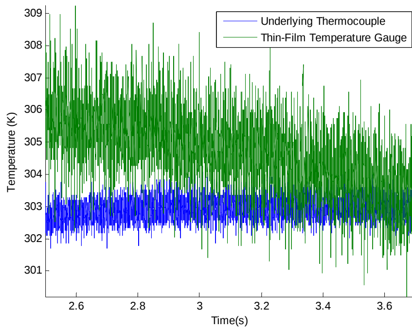
Figure 34: Sample time-resolved heat flux gauge traces: 47 % x/C BOAS
