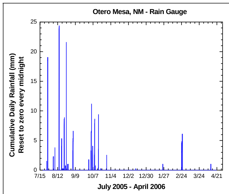
Figure 12. Precipitation data from the observation station near the RAS.
