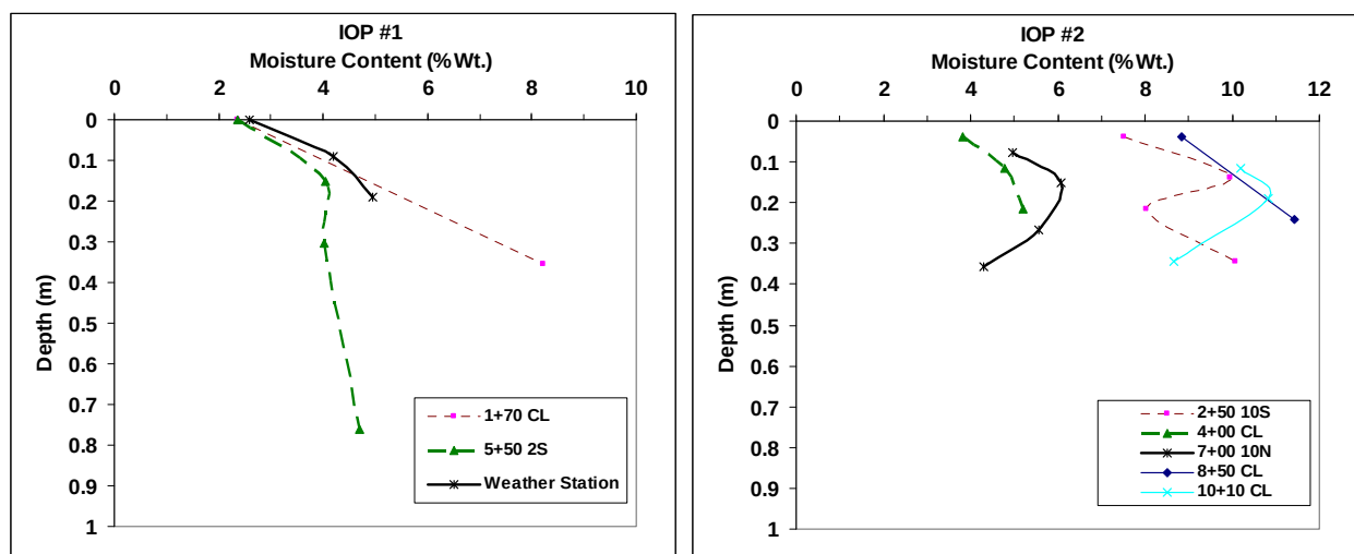
Figure 35. Soil moisture profiles using the gravimetric method from samples taken in July 2005 (IOP #1) and in October (IOP #2).
