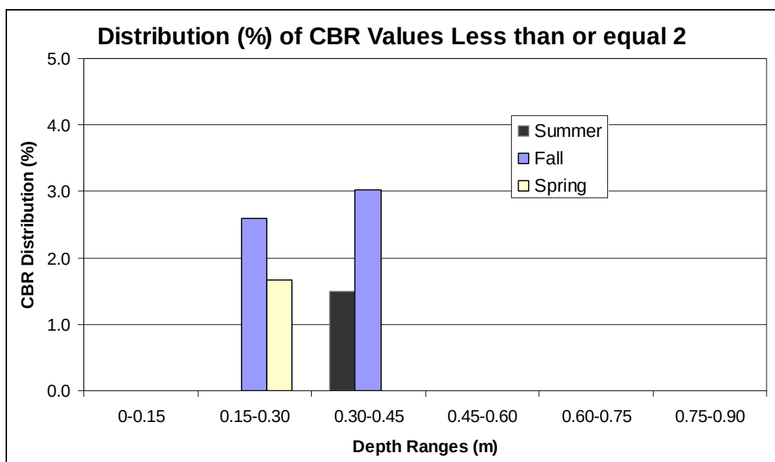
c. Number of DCP measurements with CBR value of 2 or less.
