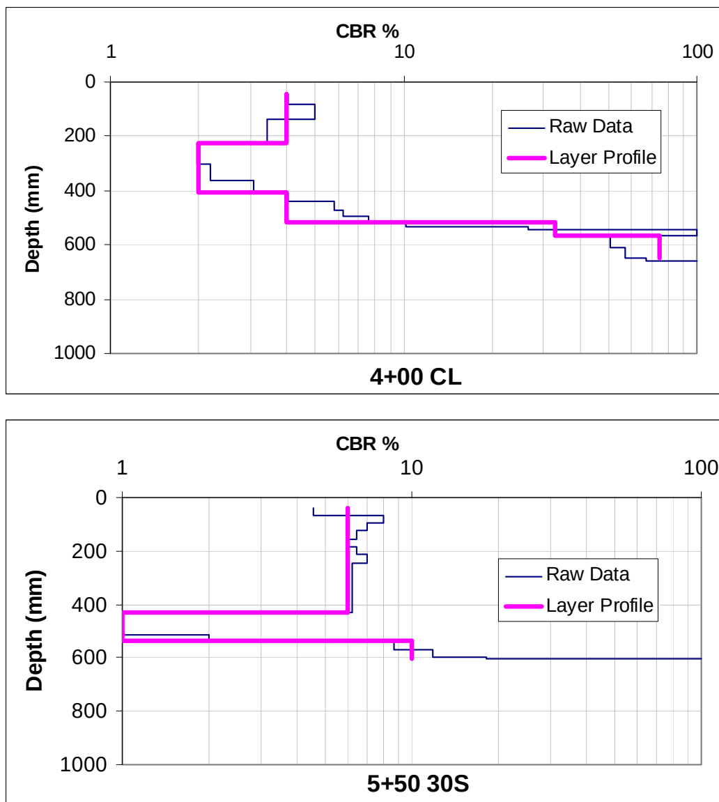
Figure 44. Selected CBR profiles showing layers with weak soil strength taken during IOP #2 at the Fort Bliss RAS.
