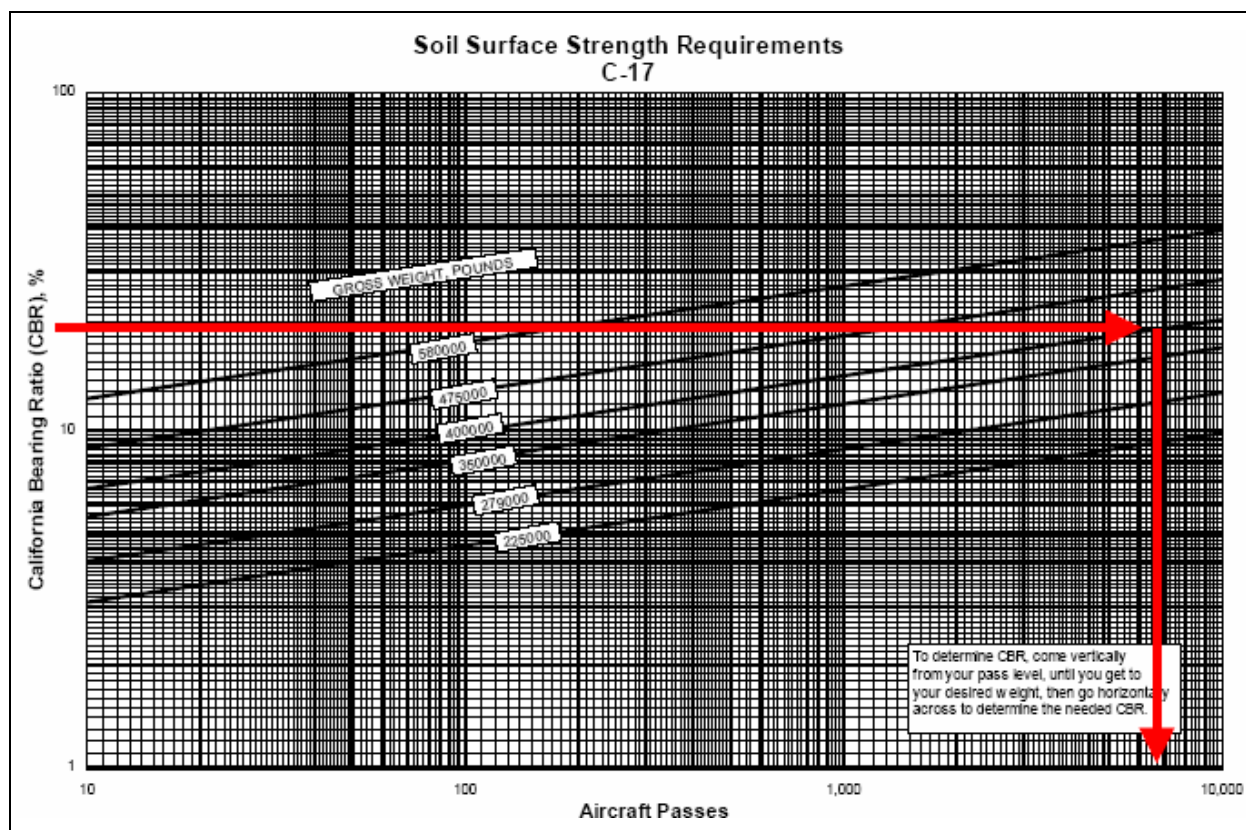
Figure 9. Sample evaluation of surface strength on semi-prepared airfield for C-17 operations.
