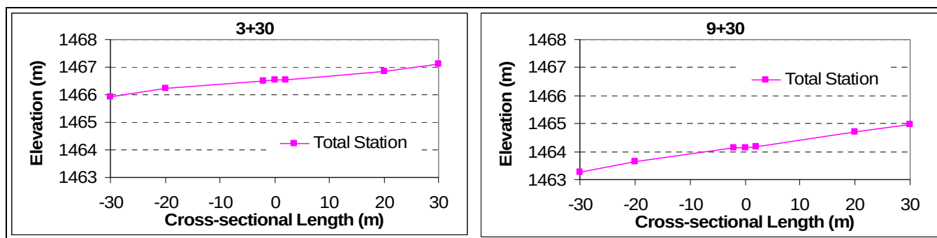
Figure 16. Typical lateral (transverse) profiles of the RAS at Fort Bliss, slope slightly to the south. Station 3+30 is 2% grade and station 9+30 is 2.8% grade.
