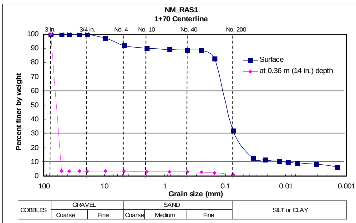
d. Results from the laboratory grain-size analysis of the soil samples.
