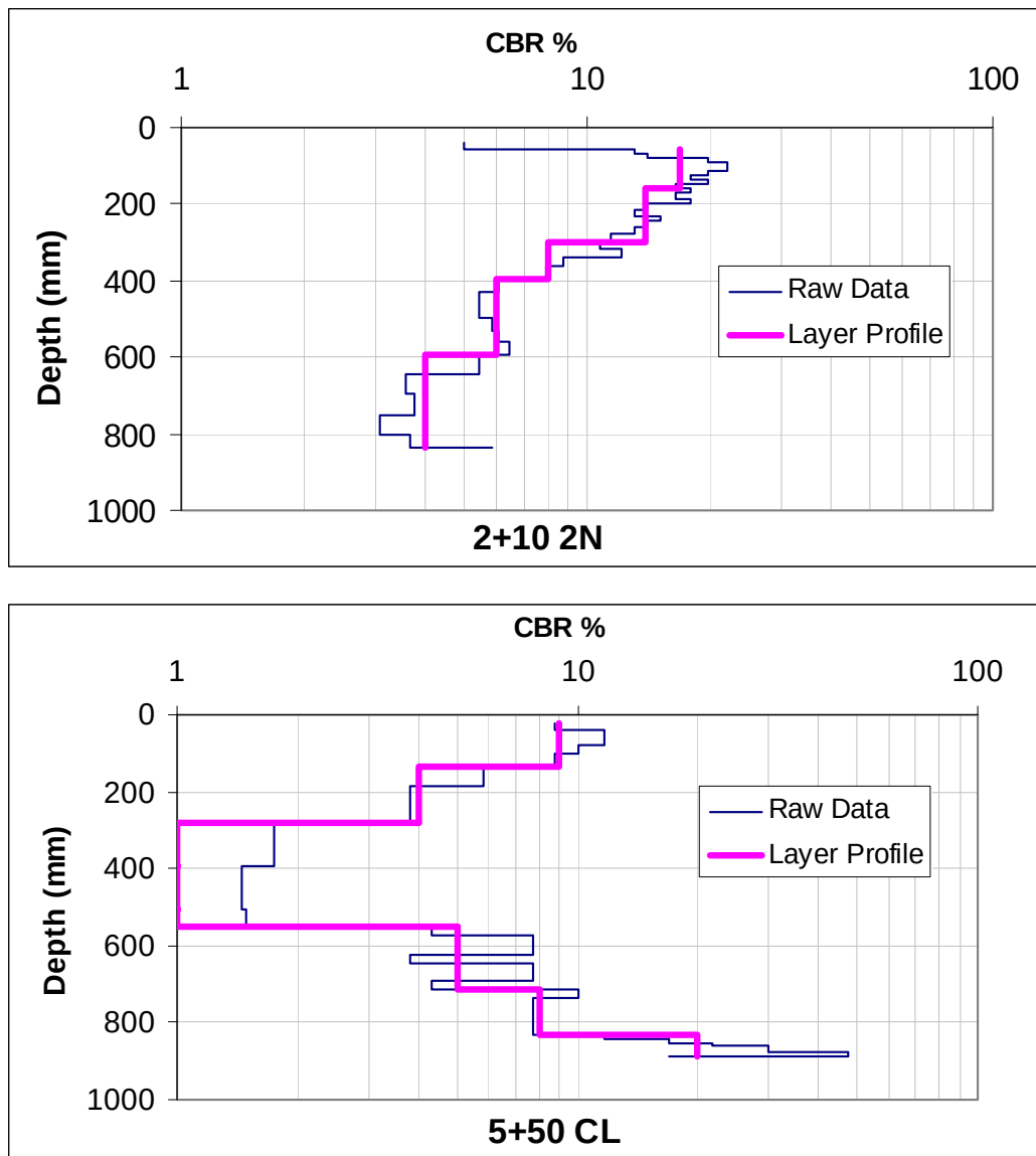
Figure 43. Selected CBR profiles showing layers with weak soil strength taken during IOP #1 at the Fort Bliss RAS.
