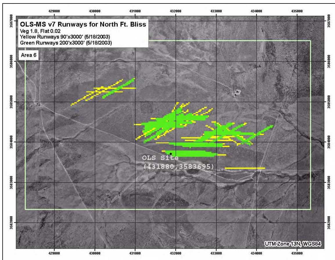
Figure 4. OLS software analysis using 200- by 3000-ft runway dimensions found many more runways (LANDSAT imagery, 18 May 2003).
