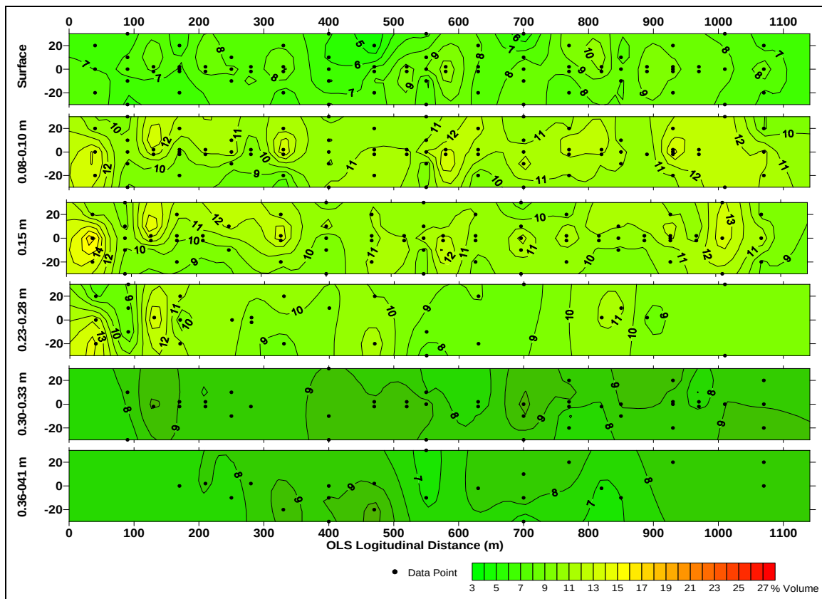
Figure 32. Profiles of soil moisture contents in % volumetric from the Dynamax ML2 taken in October 2005, as shown in contours. The dots are the sampling locations where soil moisture measurements were taken with depth in the soil.
