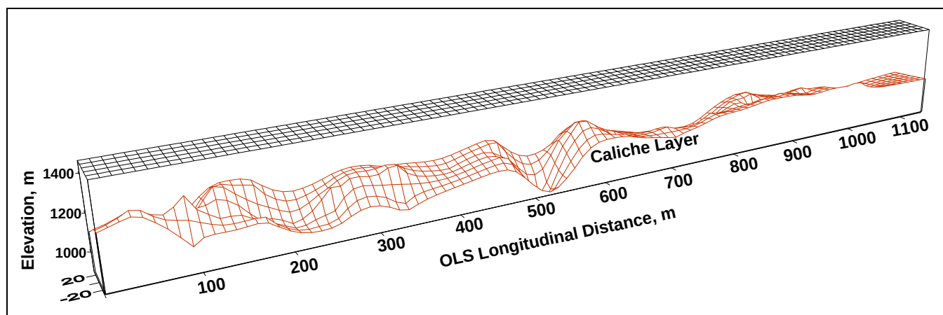
Figure 40. Profile of the topmost part of the caliche layer detected from the DCP data.
