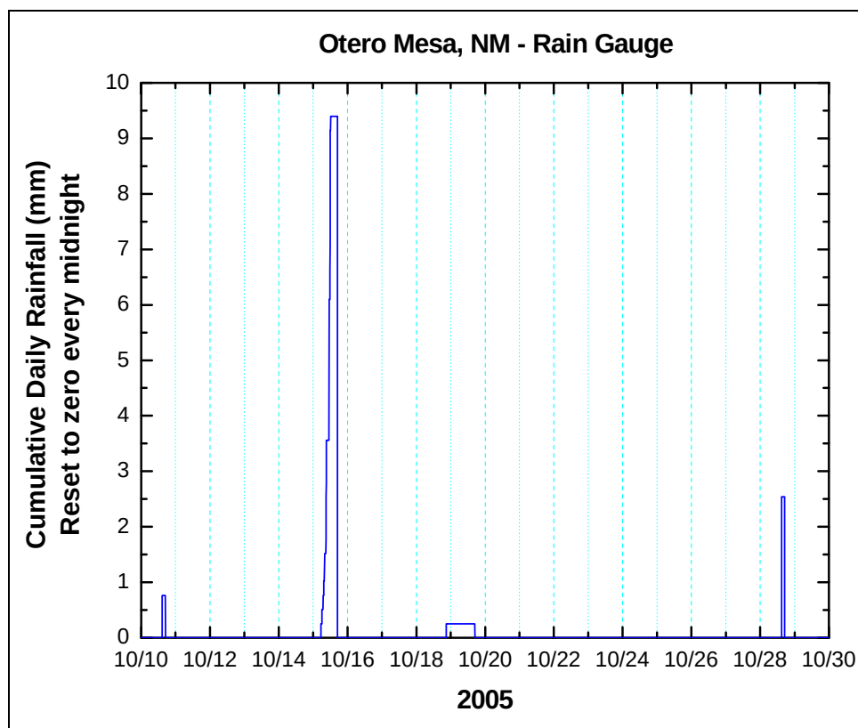
Figure 33. Precipitation observed from the weather station installed near the RAS.
