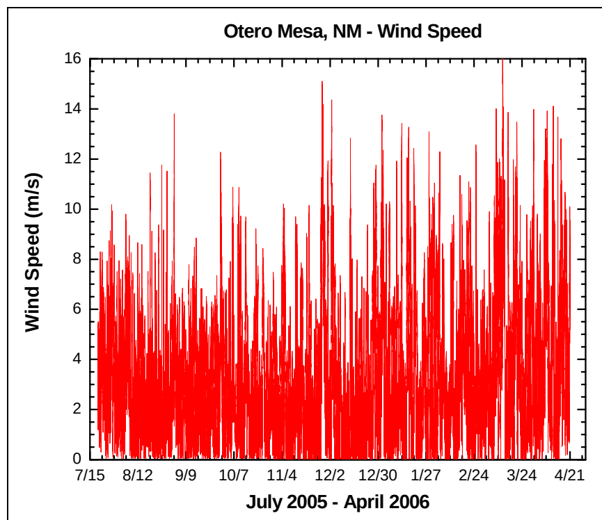
Figure 13. Wind speed observed from the weather station near the RAS averaged every five minutes for the entire monitored time.
