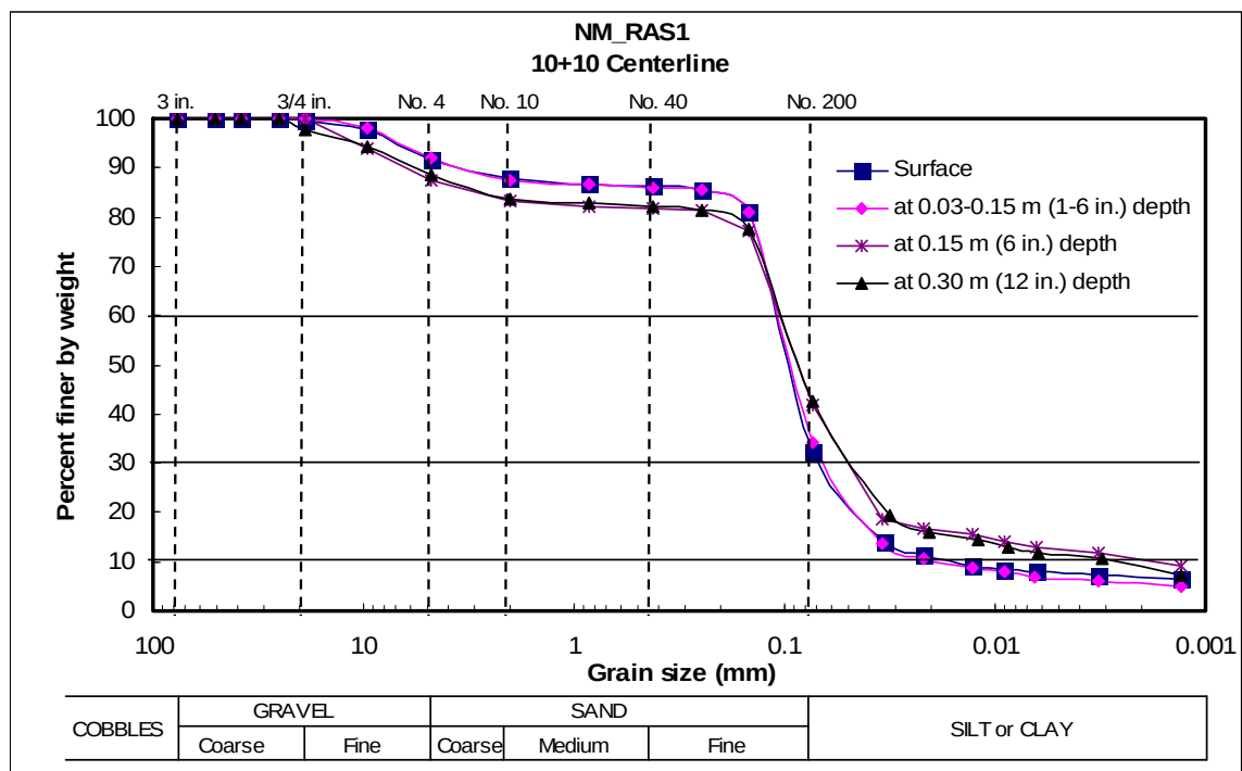
b. Results from the laboratory grain-size analysis of the soil samples.
