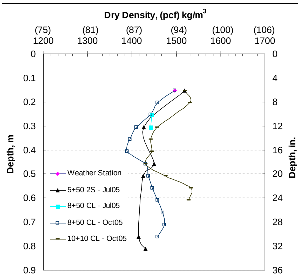
Figure 24. Soil density profiles taken using a nuclear density gage at five locations on Fort Bliss RAS.
