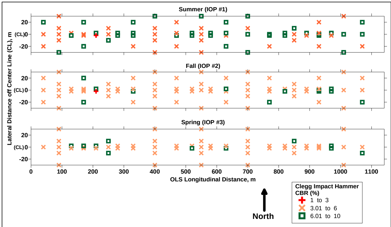
Figure 41. Soil strength for top 0.3 m (6 in.) measured from the light Clegg impact hammer expressed in CBR (%) for the Fort Bliss RAS.
