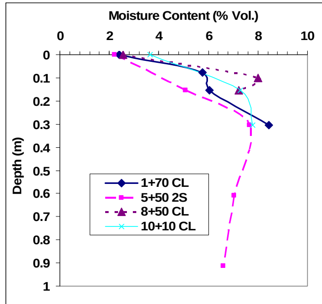
Figure 31. Average soil moisture profiles from the Dynamax ML2 probes taken during IOP #1 (July 2005)
