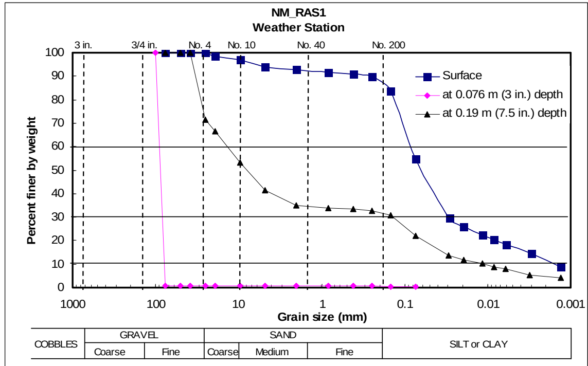
b. Results from the laboratory grain size analysis of the soil samples.
