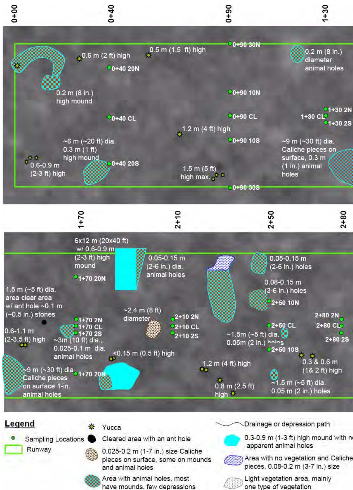
Figure 25. Symbolic representation of surface features from the visual survey along the RAS in sections.
