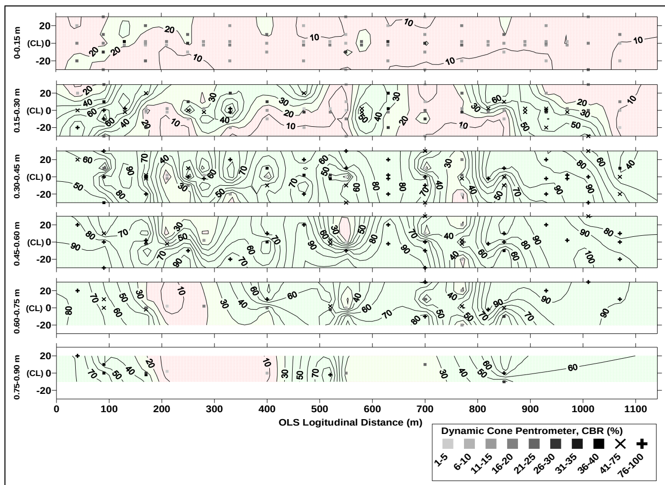
a. CBR contours for each depth range (July 2005).
