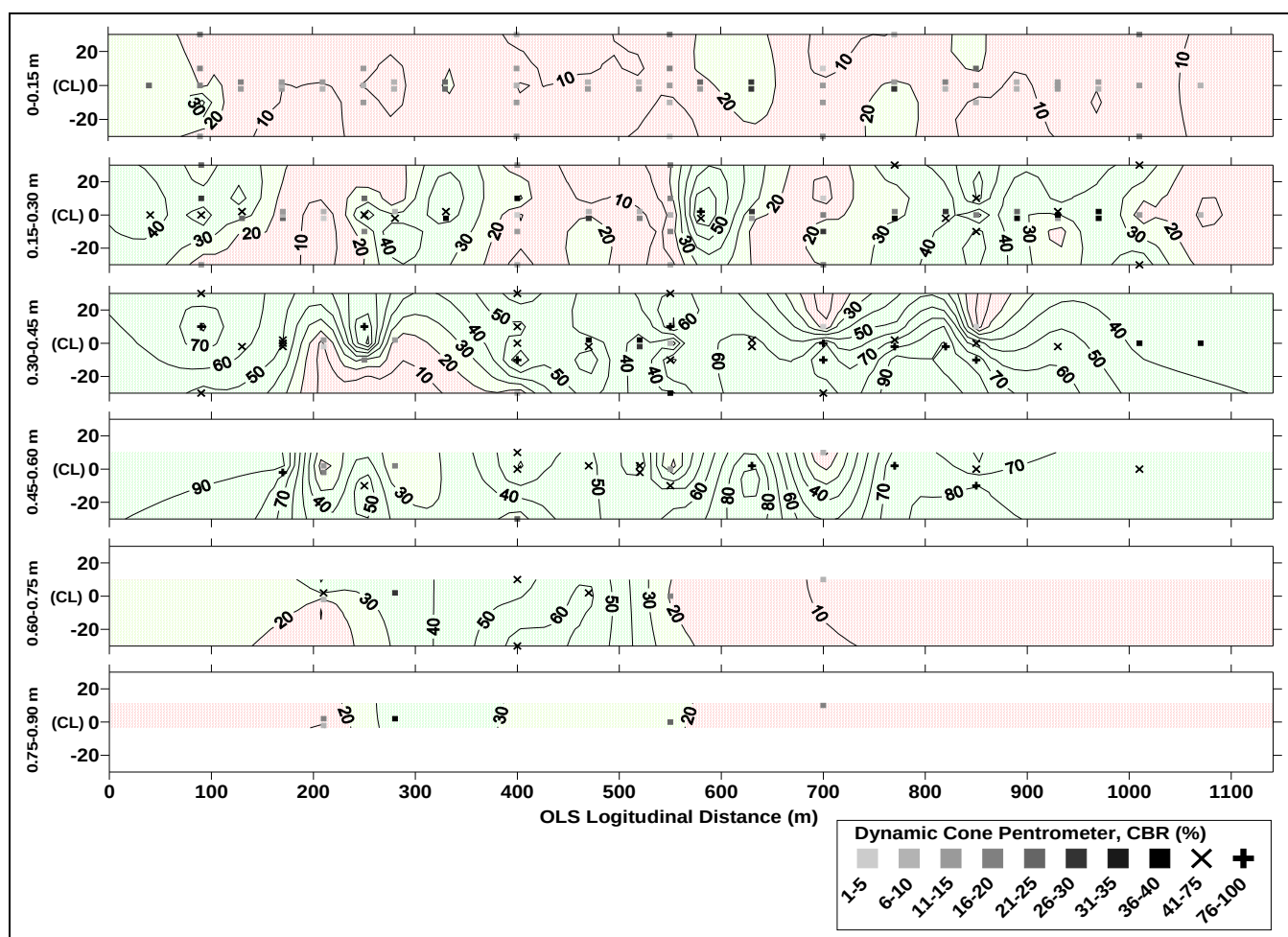
c. CBR contours for each depth range (April 2006).
