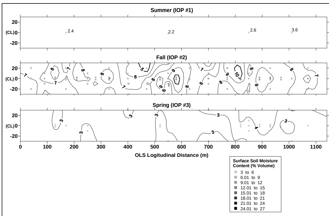
Figure 34. Surface soil moisture (in % volume) for three field visits at Fort Bliss RAS.
