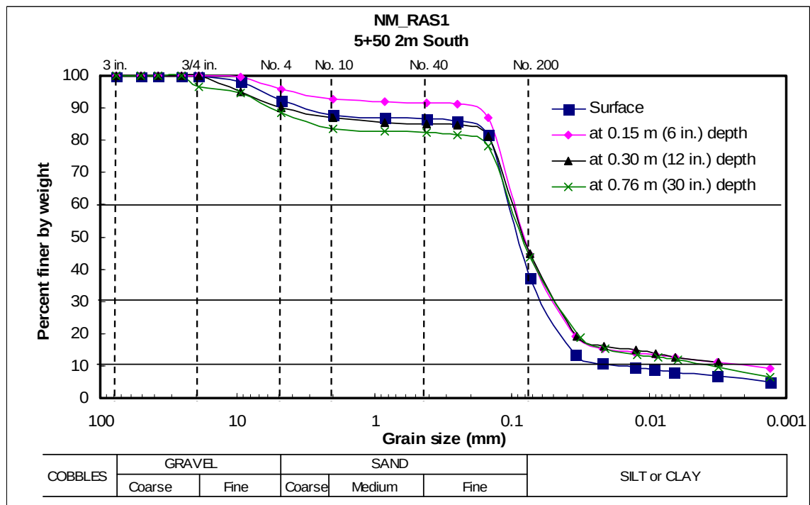
Figure 19. Soil profile at station 5+50 2S.
