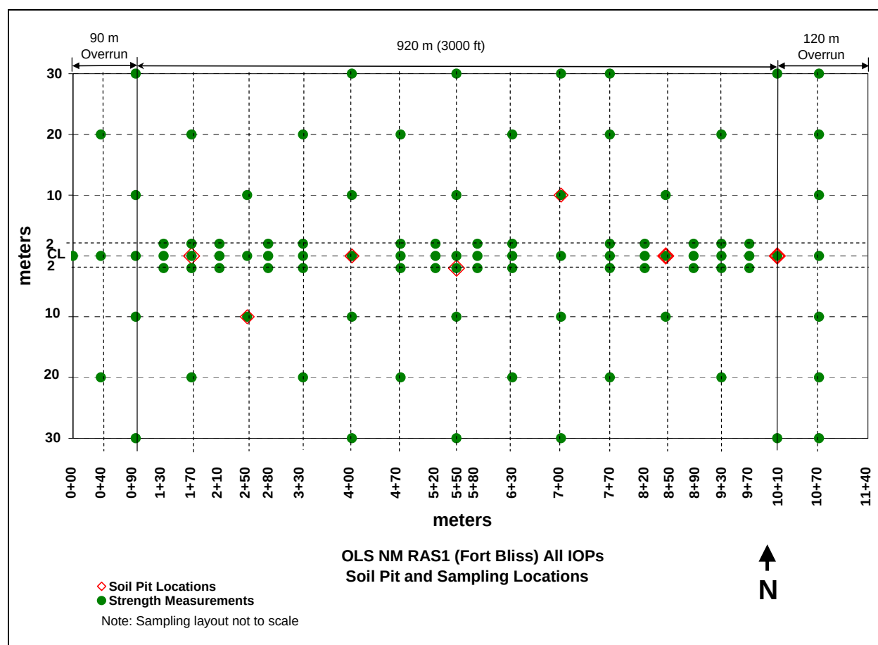
Figure 7. Sampling grid used to evaluate the RAS at Fort Bliss OLS. (Not drawn to scale.)
