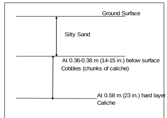
c. Soil profile in the field.
