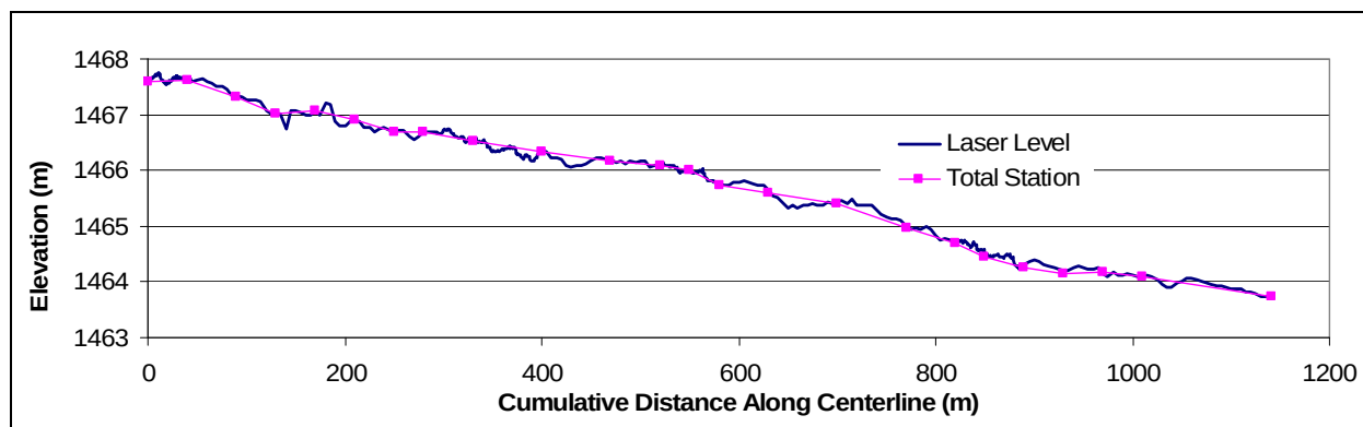
a. Elevation along the OLS centerline.
