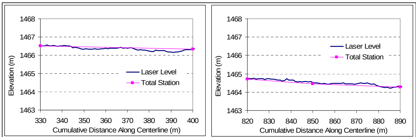
b. Surface roughness reflected from higher sampling using the laser level.
