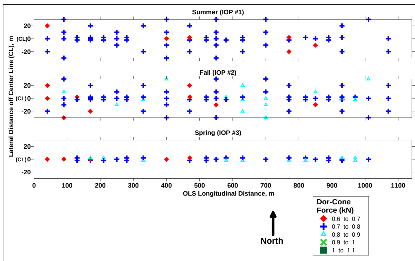
Figure 42. Calculated force indicating the surface soil strength throughout the RAS during the three IOPs.
