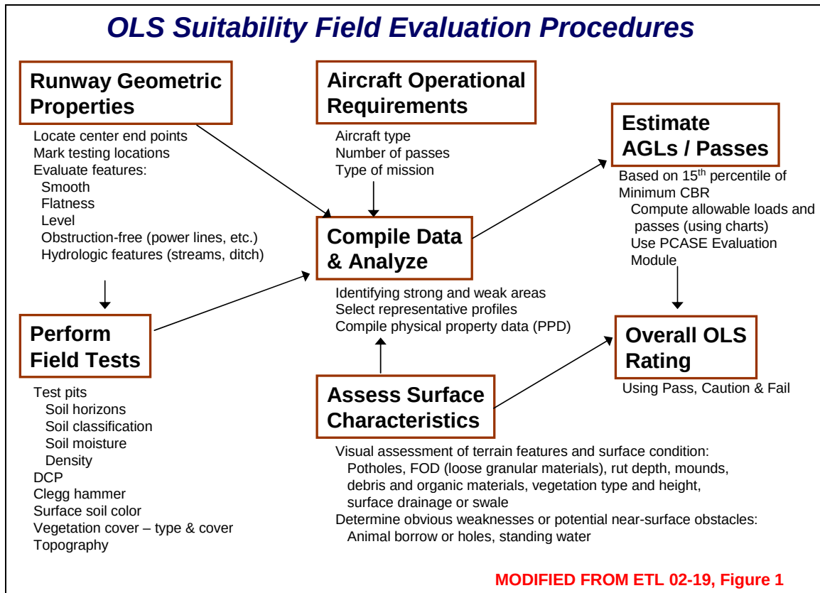
Figure 6. Procedures for determining the suitability of an OLS, modified from practice established by AFCEA in ETL 2002-19 (AFCEA 2002a).
