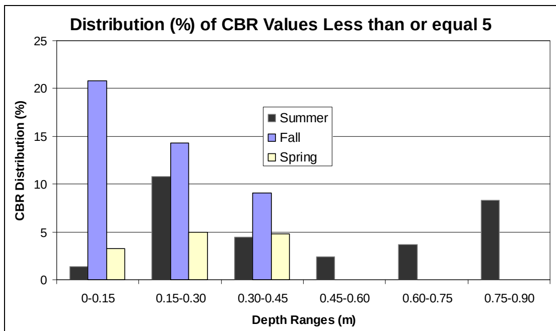
d. Number of DCP measurements with CBR values equal to or less than 5.
