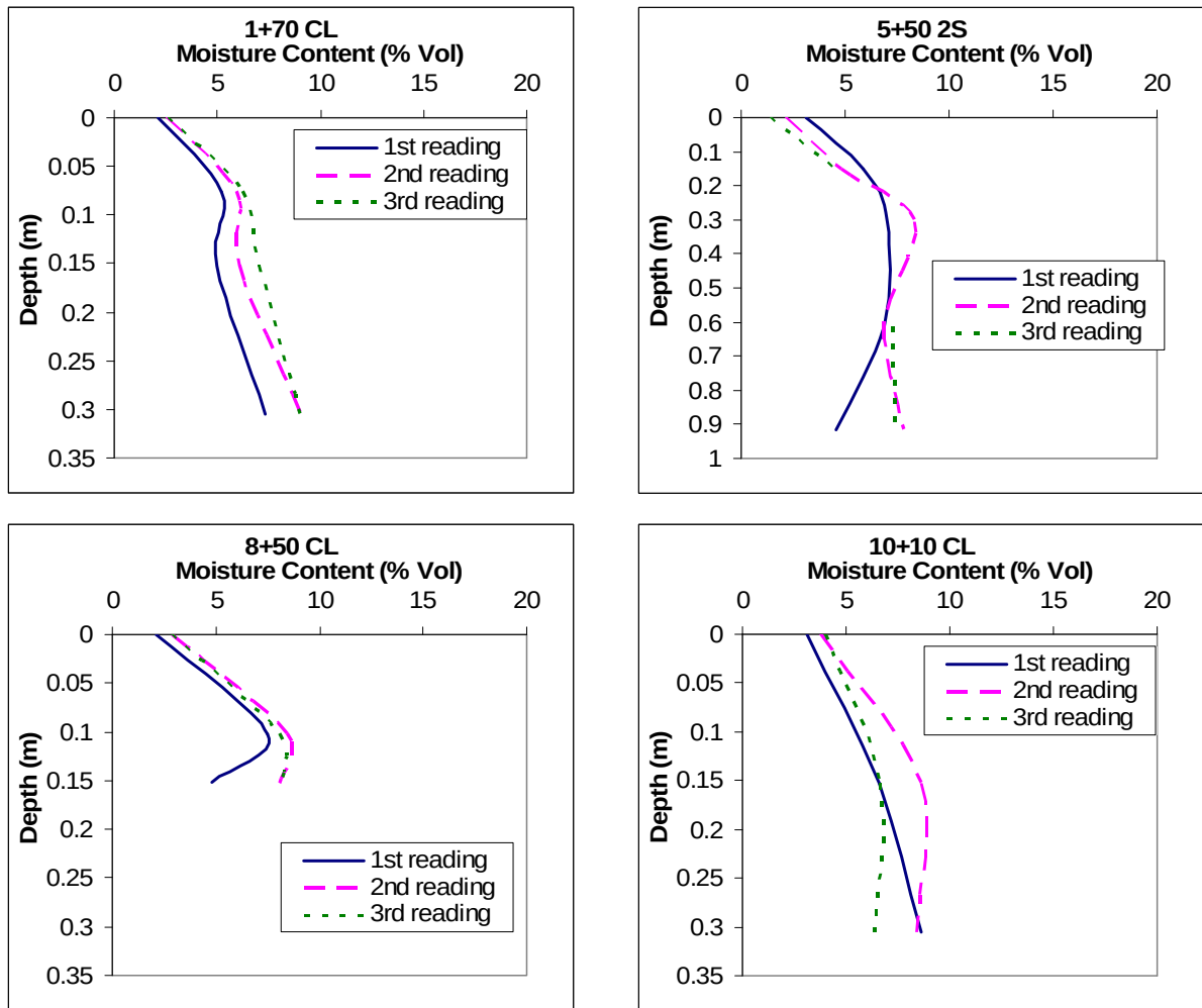
Figure 30. Moisture profiles taken from Dynamax ML2 probes during IOP #1.
