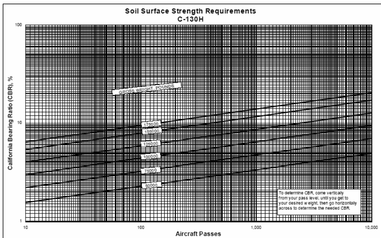
Figure 8. Soil strength on semi-prepared airfield for the C-17 and the C-130H.
