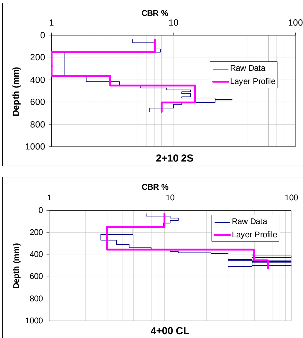
Figure 45. Selected CBR profiles showing layers with weak soil strength taken during IOP #3 at the Fort Bliss RAS.
