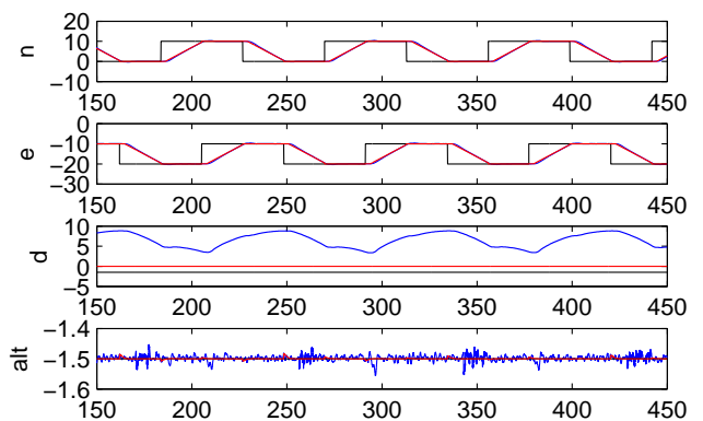
Fig. 5. North, East, Down, and Altitude Position vs. Time: Blue line is the actual vehicle trajectory, black line is the command, and the red line is filtered command
