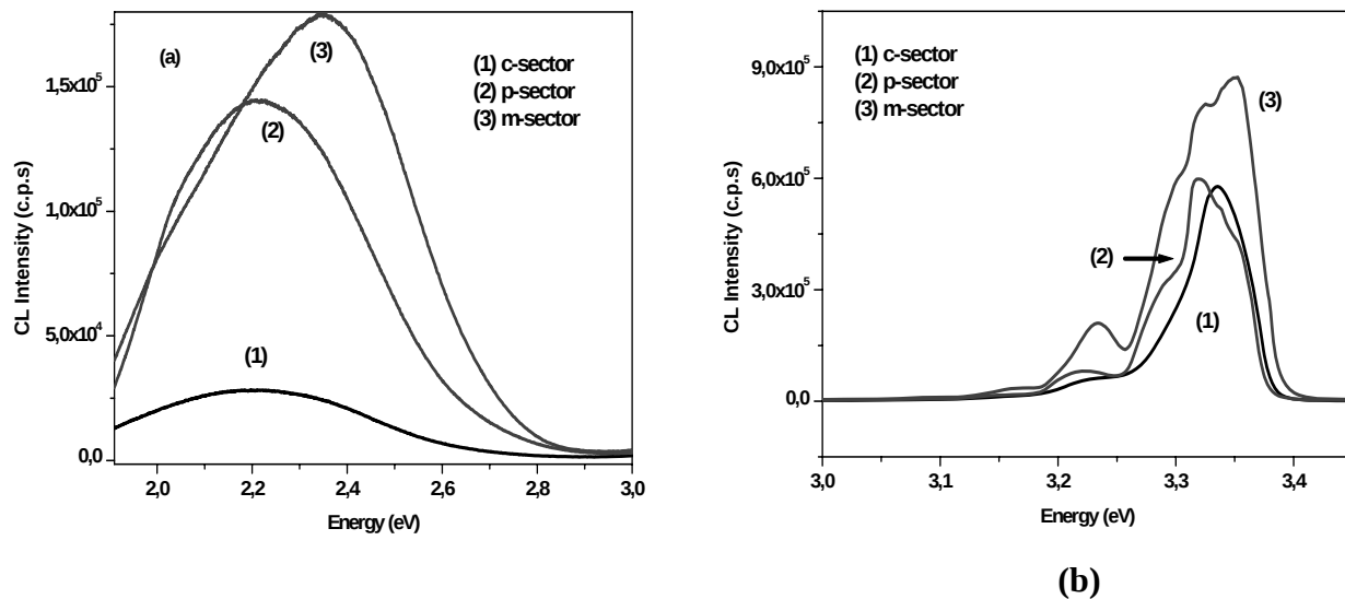
(a) Figure 4. CL spectra at different growth sectors. (a) visible range, (b) UV range.
