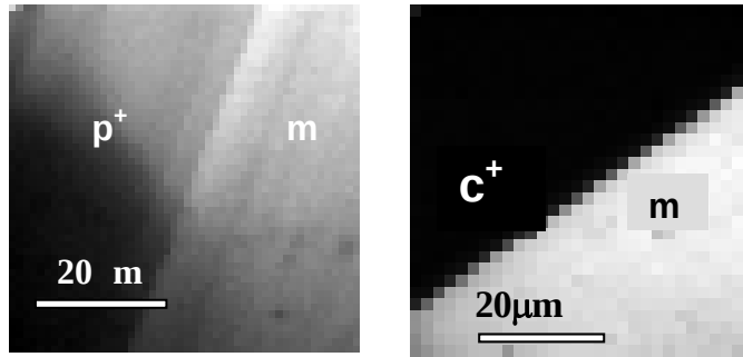
Figure 5. Monochromatic images ( visible luminescence) of the boundaries between the growth sectors, showing weak contrast between pa and ma and strong contrast between m and c sectors.
