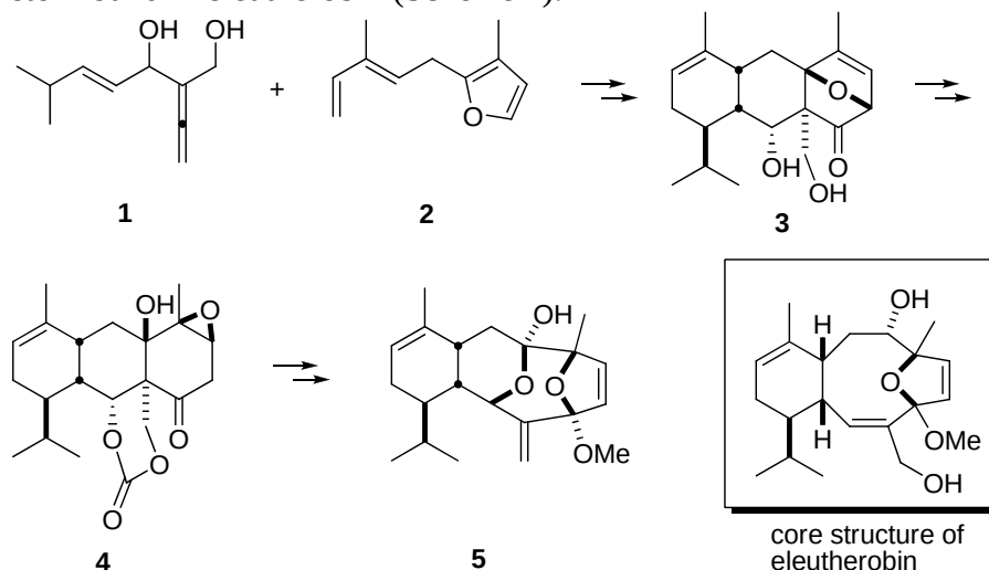
Scheme 1. Previous approach
