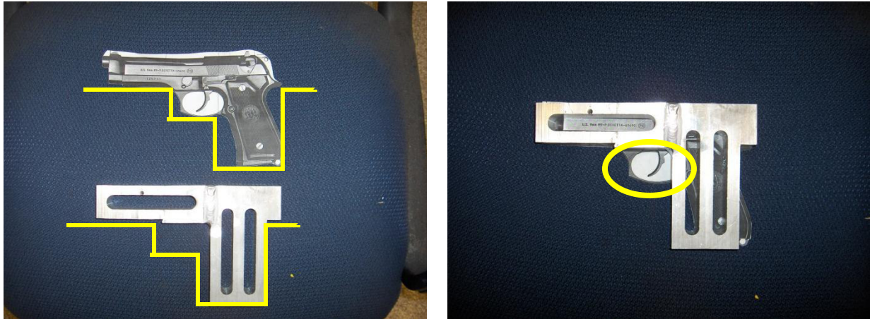
Figure 13. Comparison of (a photograph of) M9 with a dummy item, showing how items fit into foam cutout. Dummy items had no trigger to prevent them from sliding within the case.
