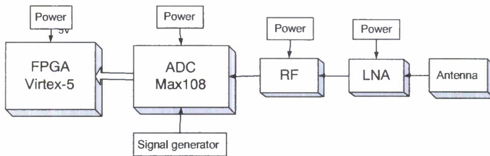
Figure 6.13: The architecture of the Test-bed receiver
