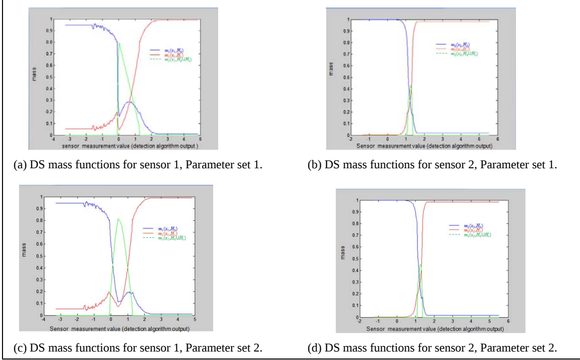
Figure 7. DS mass functions (including uncertainty function, in green) found by the particle swarm for parameter sets shown in figure 6.
