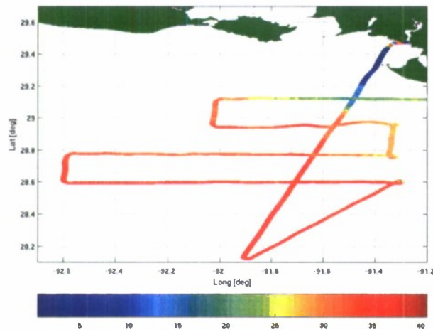
Fig. 5. Salinity map predicted by the optical data for the morning flight on May 10, 2007.
