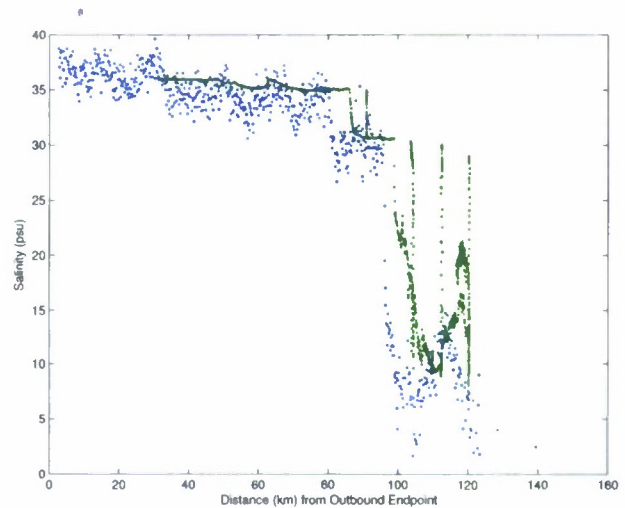
Fig. 2. R/V Pelican (green) and STARRS (blue) salinity along the outbound flight leg. STARRS data is from the afternoon flight. The ship was at the salinity front when the aircraft flew over it. The ship covered the distance shown in approximately 12 hours while the aircraft covered it in less than 45 minutes.
