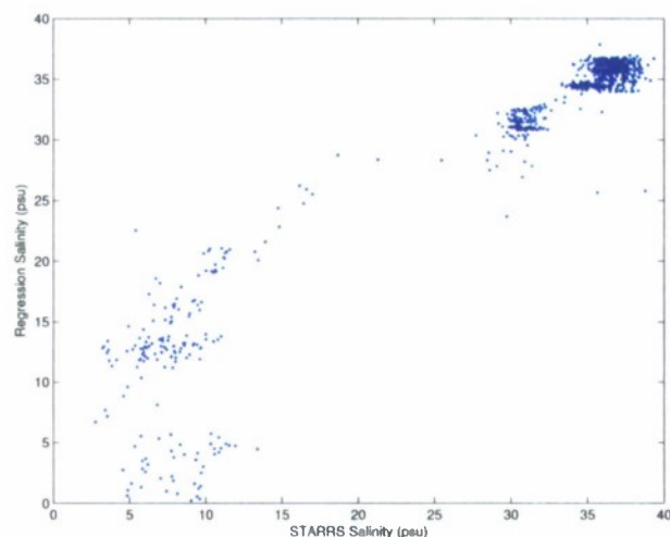
Fig. 4. Regression results for salinity based on the linear fit to (Band5/Band2) and (Band5/Band6) values along the outbound leg for the morning flight.
