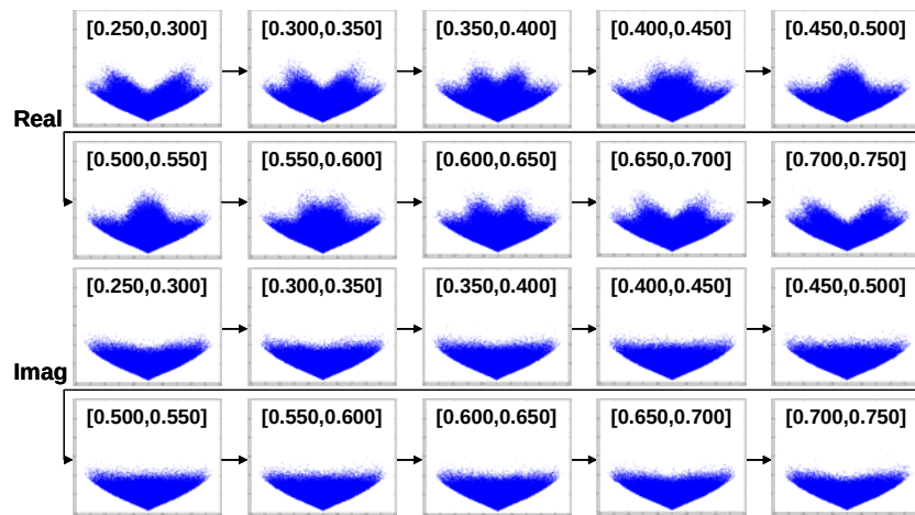
Figure 2.13 – Bandpass FFT Real and Imaginary Plots
