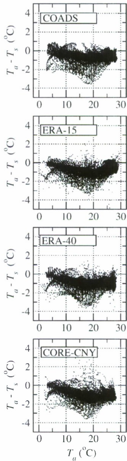
Fig. 3. Scatter plots of near-surface air temperature ( T_a ) versus T_a - T_s based on annual mean values (see Fig. 1), each at 1^\circ bins over the global ocean.
