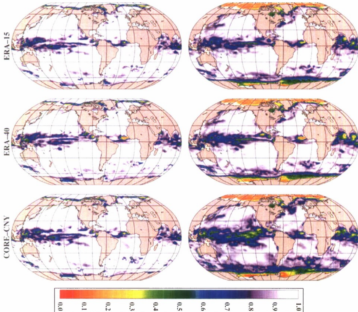
(a) Correlation: HYCOM vs NOAA SST
