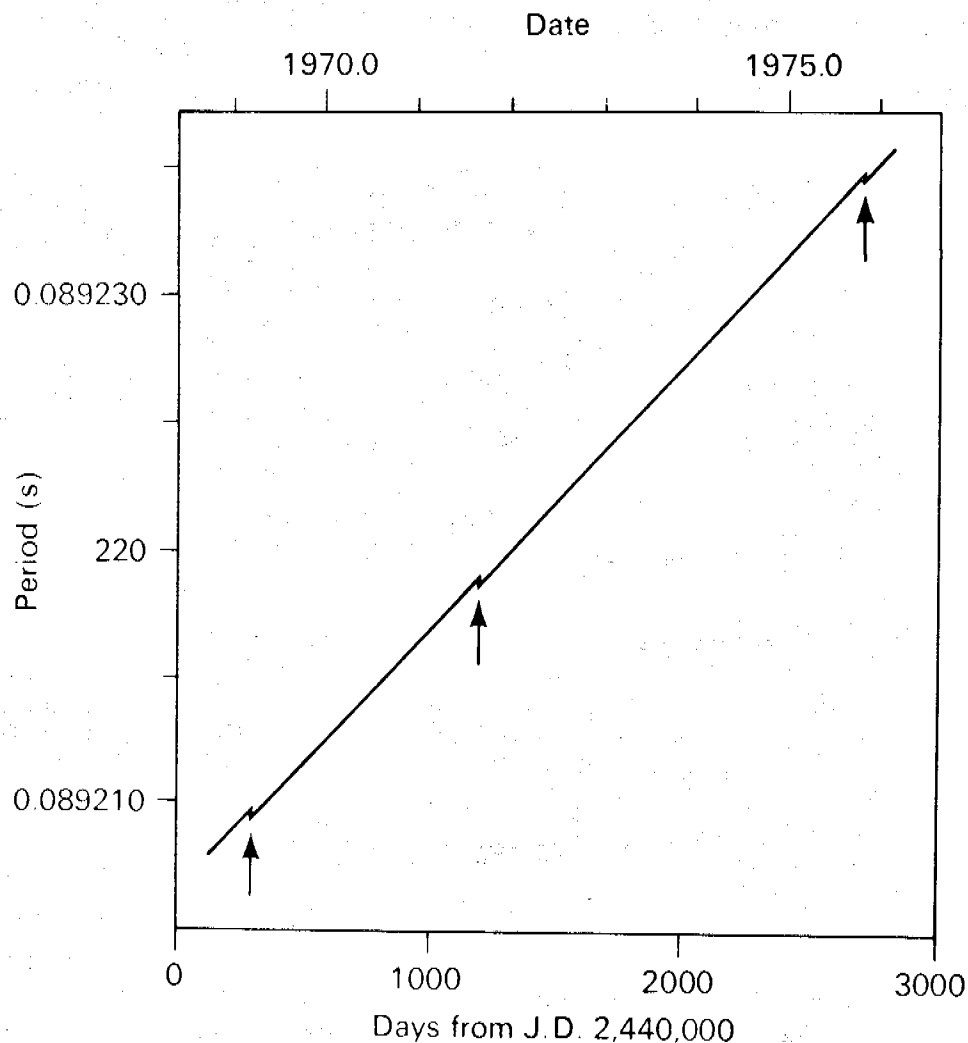
Figure 4. Variations in the period of the Vela pulsar, PSR0833-45, from 1968 to 1976, showing three discontinuous steps in the regular increase of the period. [Used from Manchester and Taylor, 1977 (Figure 6-4, p. 114), with permission.]
