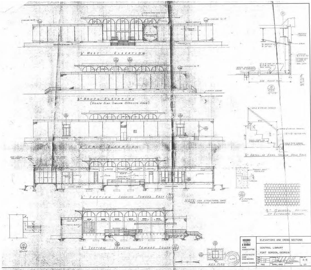
Plan 2 – elevations and cross sections, April 1965.
