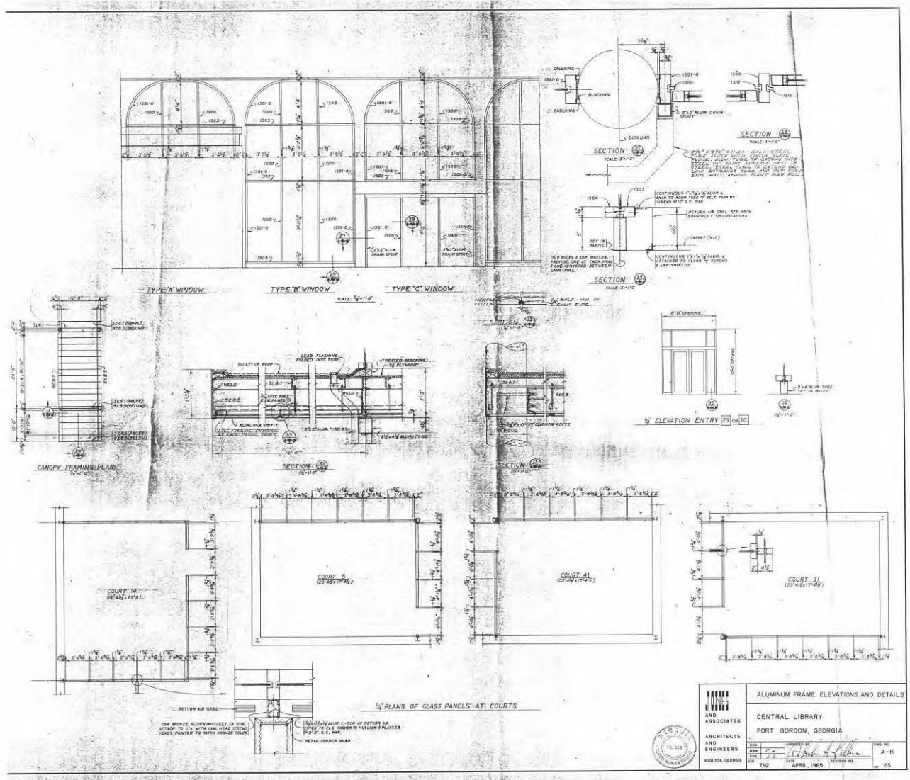
Plan 3 – aluminum frame elevations and details, April 1965.
