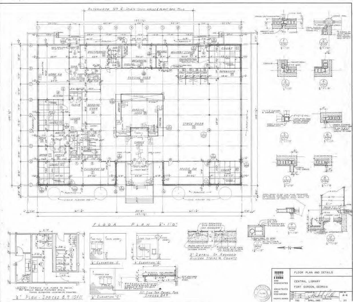
Plan 1 – floor plan and details, April 1965.
