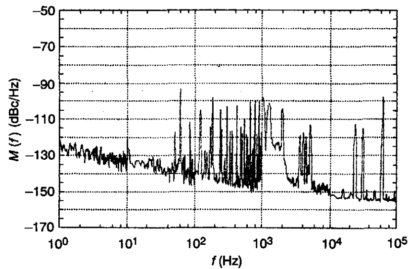
Figure 3. Reference oscillator AM noise.
