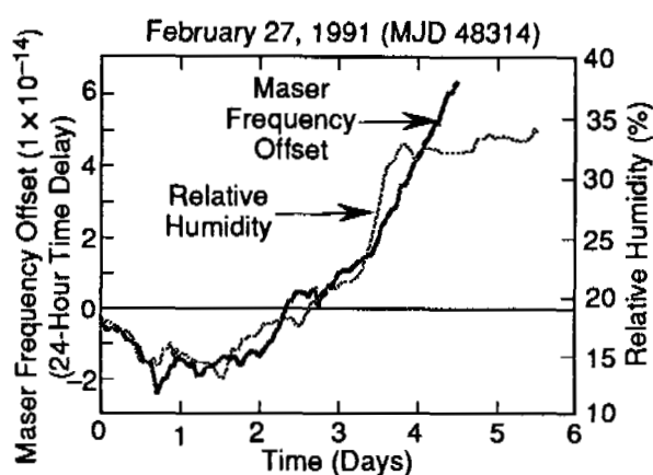
Figure 5B. Maser Frequency Offset and Relative Humidity Versus Time. (Note: The frequency offset curve has been delayed by 24 hours with respect to the relative humidity curve.)
