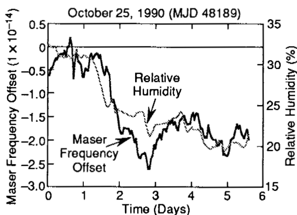
Figure 3B. Maser Frequency Offset and Relative Humidity Versus Time.
