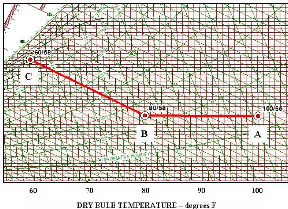
Figure 23. Psychrometrics of indirect/direct evaporative cooling.
