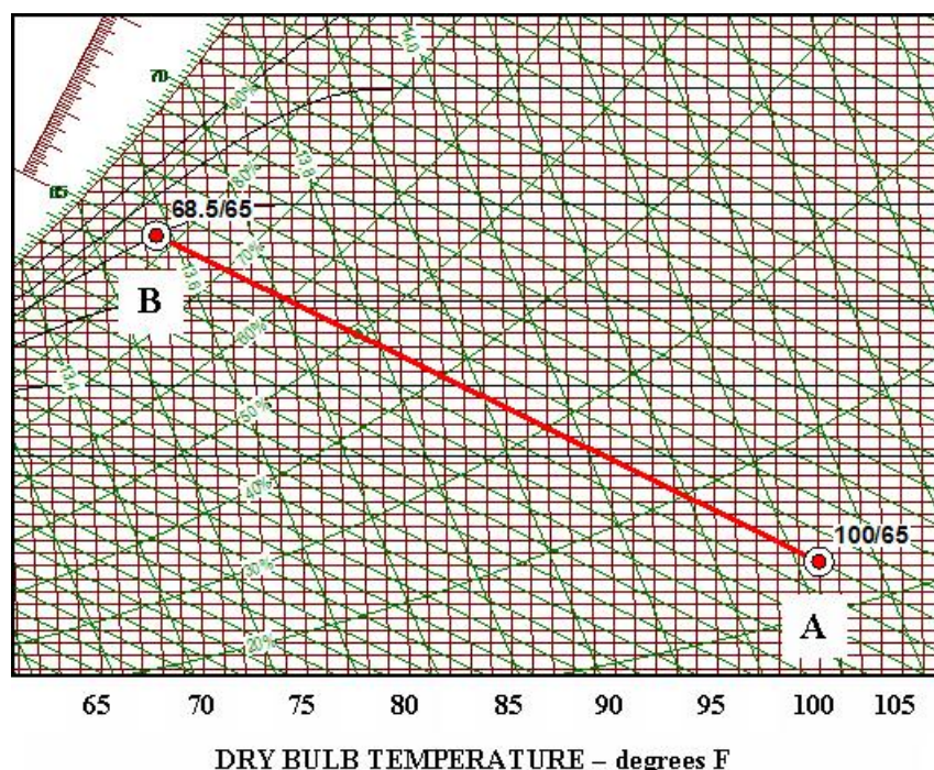
Figure 19. Psychrometrics of 90 percent effective direct evaporative cooling.
