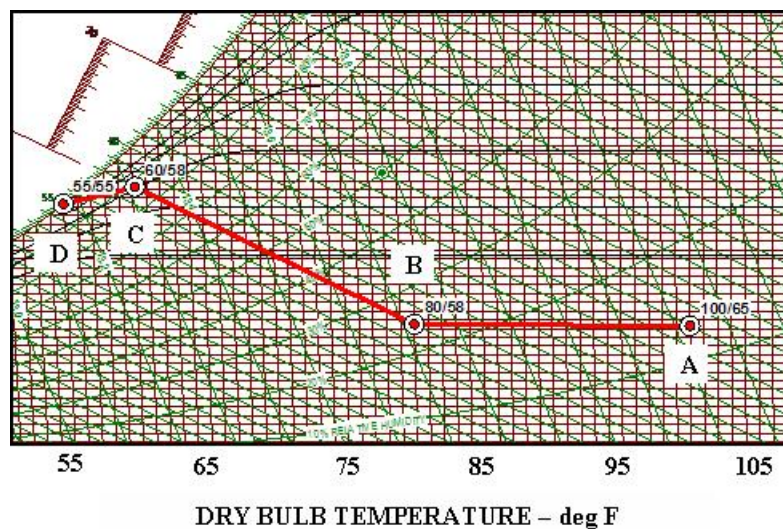
Figure 25. Psychrometrics of indirect/direct/DX cooling.
