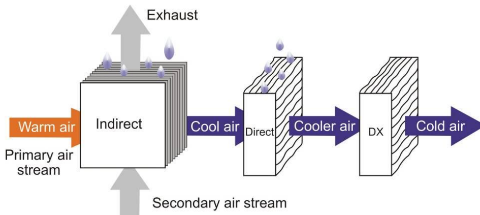
Figure 24. Diagram of a three-stage indirect/direct/DX cooler.
