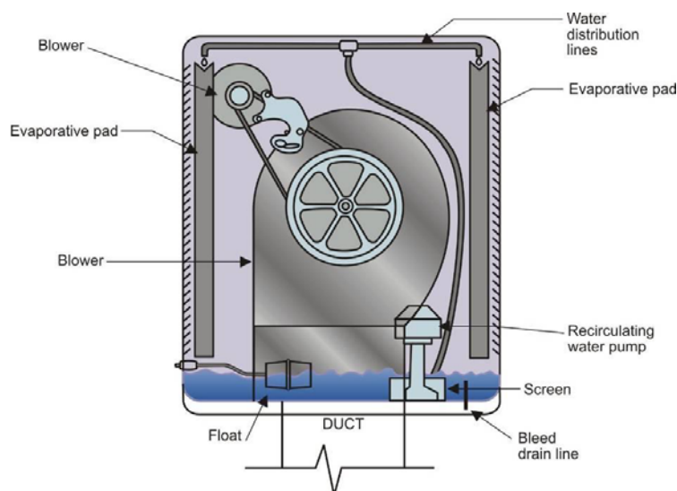
Figure 18. Diagram of a direct evaporative cooler.
