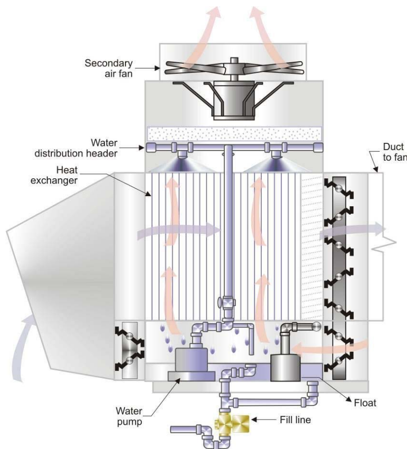
Figure 20. Diagram of an indirect evaporative cooler.
