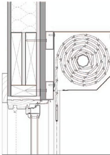
Figure 11. Installation of shade outside window.
