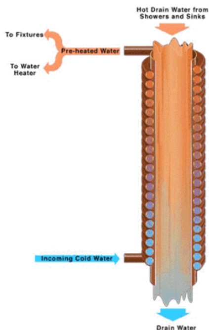
Figure 32. Shower drain heat recovery unit.
