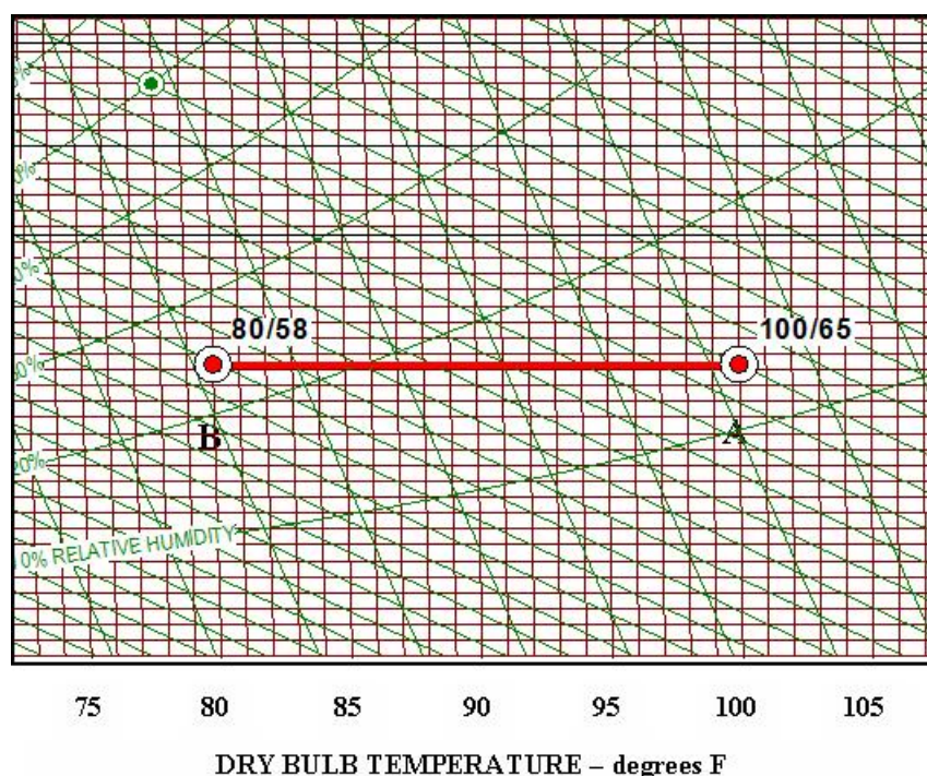
Figure 21. Psychrometrics of 75 percent effective indirect evaporative cooling.
