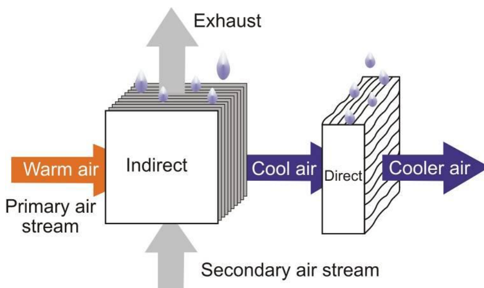
Figure 22. Diagram of a hybrid indirect/direct evaporative cooler.
