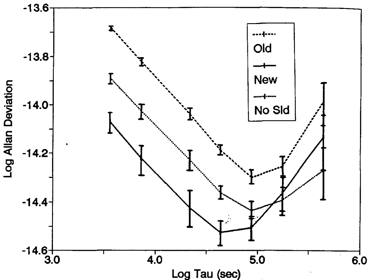
FIG. 13. FREQUENCY STABILITIES OF TIMESCALES COMPUTED WITH THE OLD WEIGHTS, THE NEW WEIGHTS, AND THE NEW WEIGHTS BUT WITHOUT THE SLIDING RELATION
