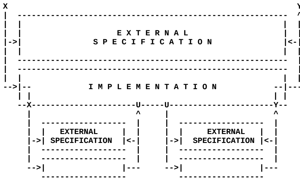
Figure 1: Gypsy Software System Structure
