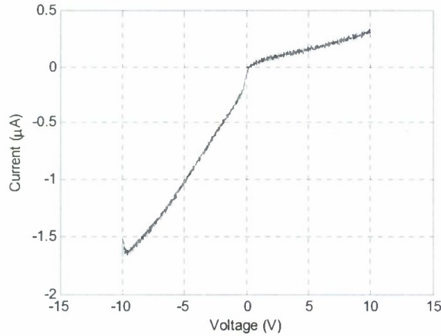
Figure 7: IV curve for quantum dot waveguide indicating minimal leakage current within the range of +10 to -10V.
