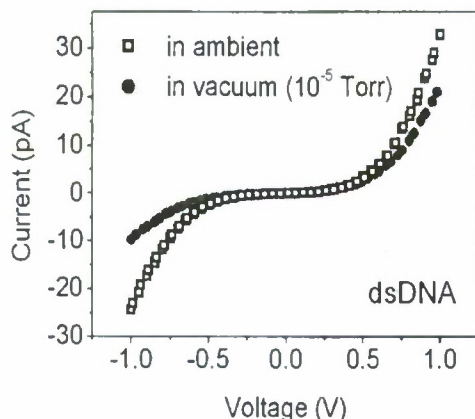
Figure 5. Current flow at room temperature through single dsDNA molecule of 80 base pair length attached between SWNT nanoelectrodes, in ambient and in vacuum conditions.
