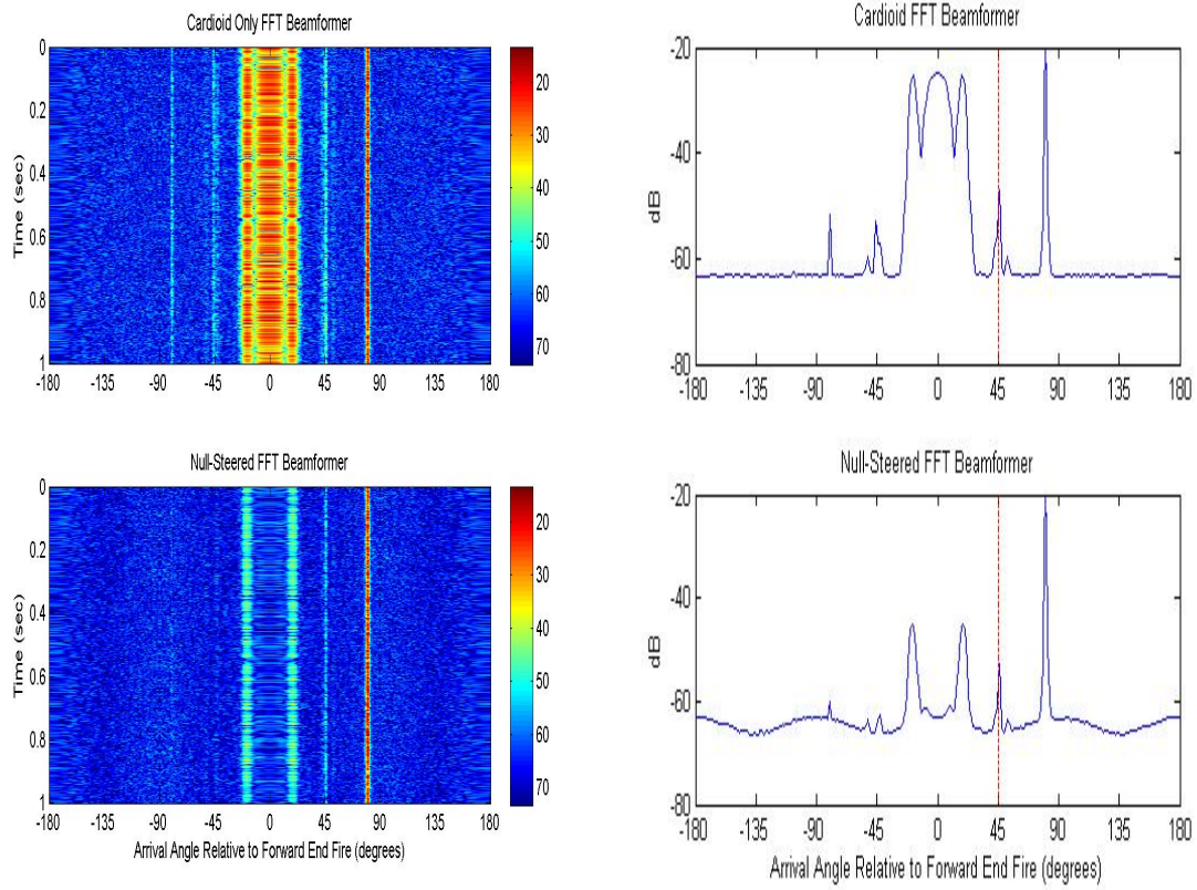
Figure 46. Cardiod and Null-Steered Comparison of Source 1 (45°) and Loud Interferer (80°) with Tow-Ship (0°) in Noisy Environment
