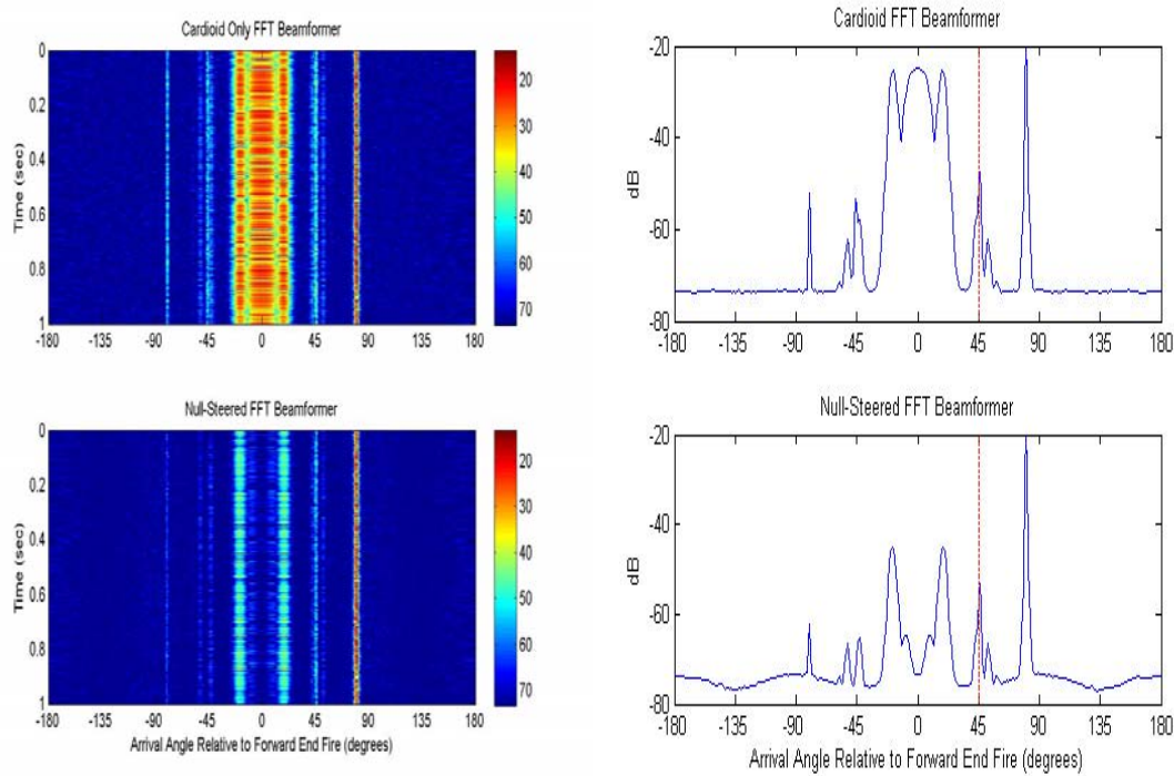
Figure 45. Cardioid and Null-Steered Comparison of Source 1 (45°) and Loud Interferer (80°) with Tow-Ship (0°)
