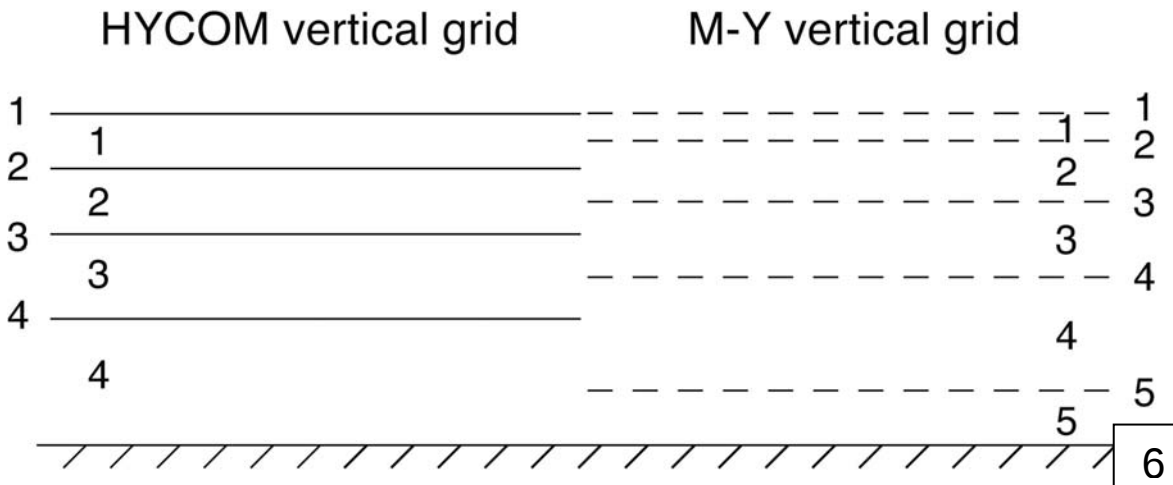
Figure 2: Side-by-side comparison of the HYCOM 2.2 vertical grid and the M-Y vertical grid used to perform the local solutions of (94) and (95).
