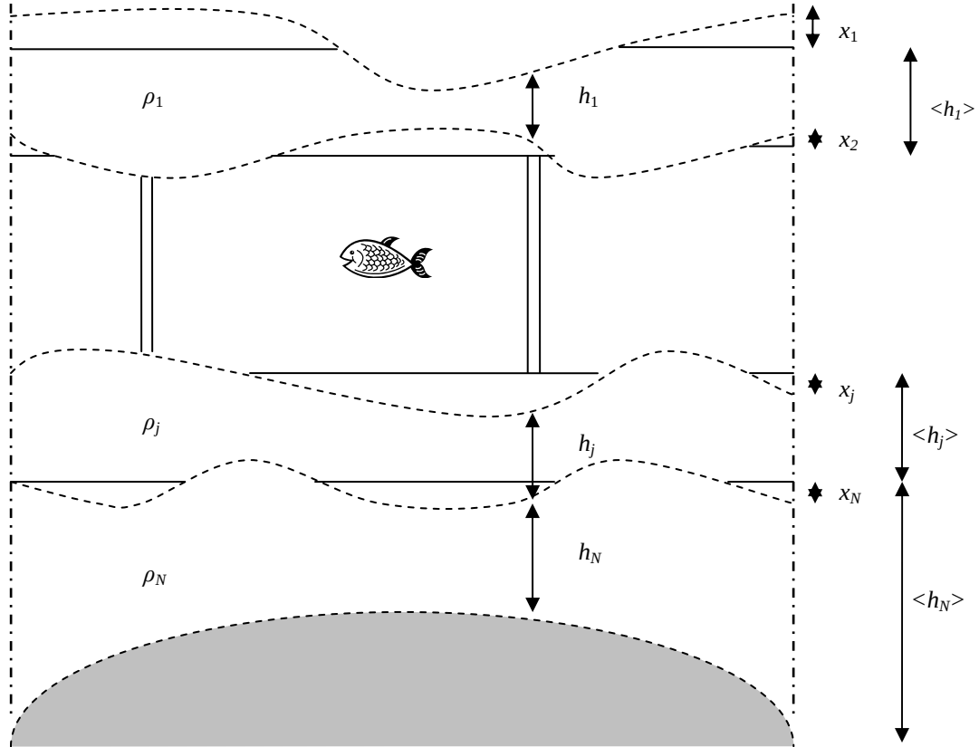
Figure 5: Vertical discretization of the multilayer ocean.
