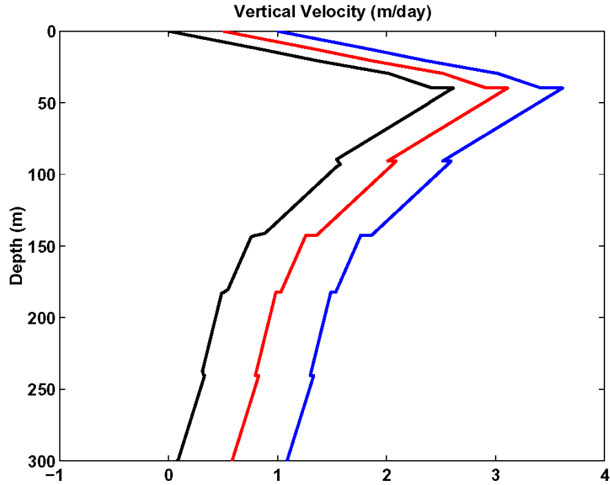
Figure 4. Vertical profile of W in m/day calculated from re-gridding horizontal velocity components onto a Cartesian coordinate system and vertically integrating (134) (black line) for the upper 3000 m (top) and the upper 300 m (bottom). Also shown are profiles calculated from (141) (red line) and from (155) (blue line), each displaced 0.5 m/day to the right.
