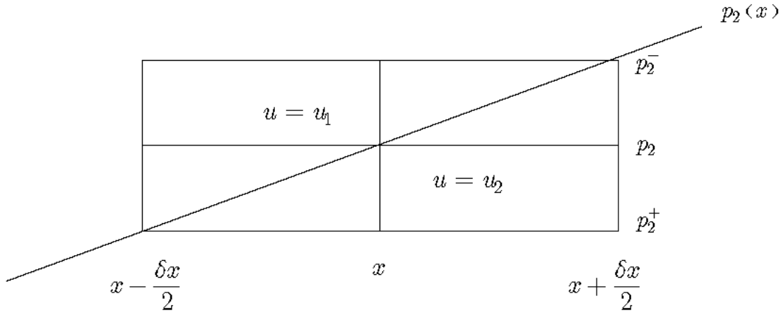
Figure 3: Vertical integration of the continuity equation (134) in a non-Cartesian grid across a model interface that slopes in the x direction.
