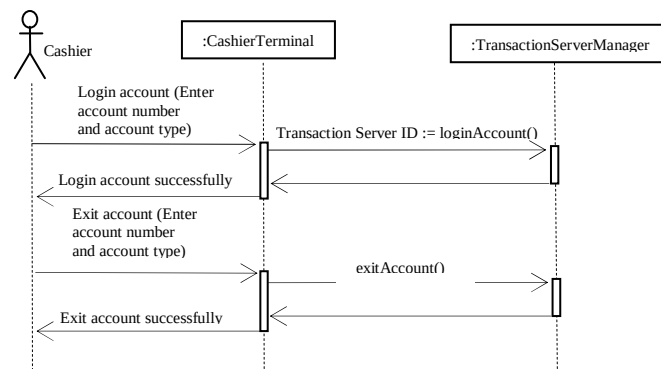
Figure C.3 Sequence Diagram of Login-exitAccount_Cashier
