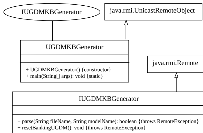
Figure 7.18 Class Diagram for UGDMKBGenerator
