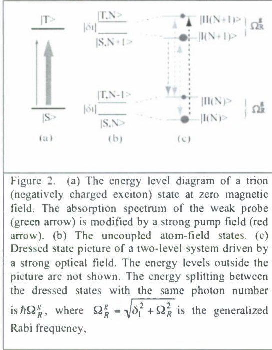
Figure 2 shows the basic approach of the experiment. A strong optical field drives the trion transition. A weak probe field then measures the resulting absorption spectrum. On the right of Fig. 2 is the dressed atom picture discussed in the previous report. When the pump detuning is large compared to the line width, level shifts are observed.
