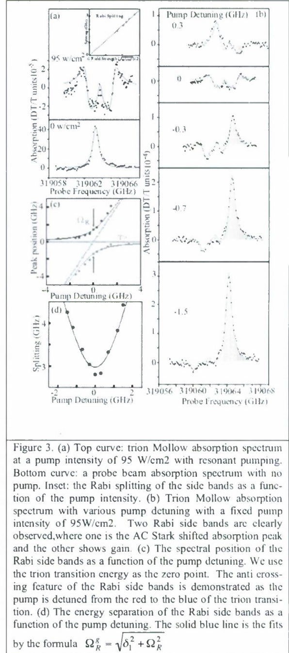
Figure3 shows the essential results of this experiment. In Fig. 3a, the basic two side bands are revealed at high power with
