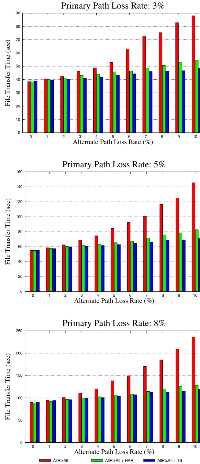
Figure 2.7: AllRtxAlt and its extensions at {3, 5, 8}% primary path loss
