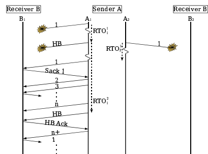
Figure 3.8: Timeout scenarios
