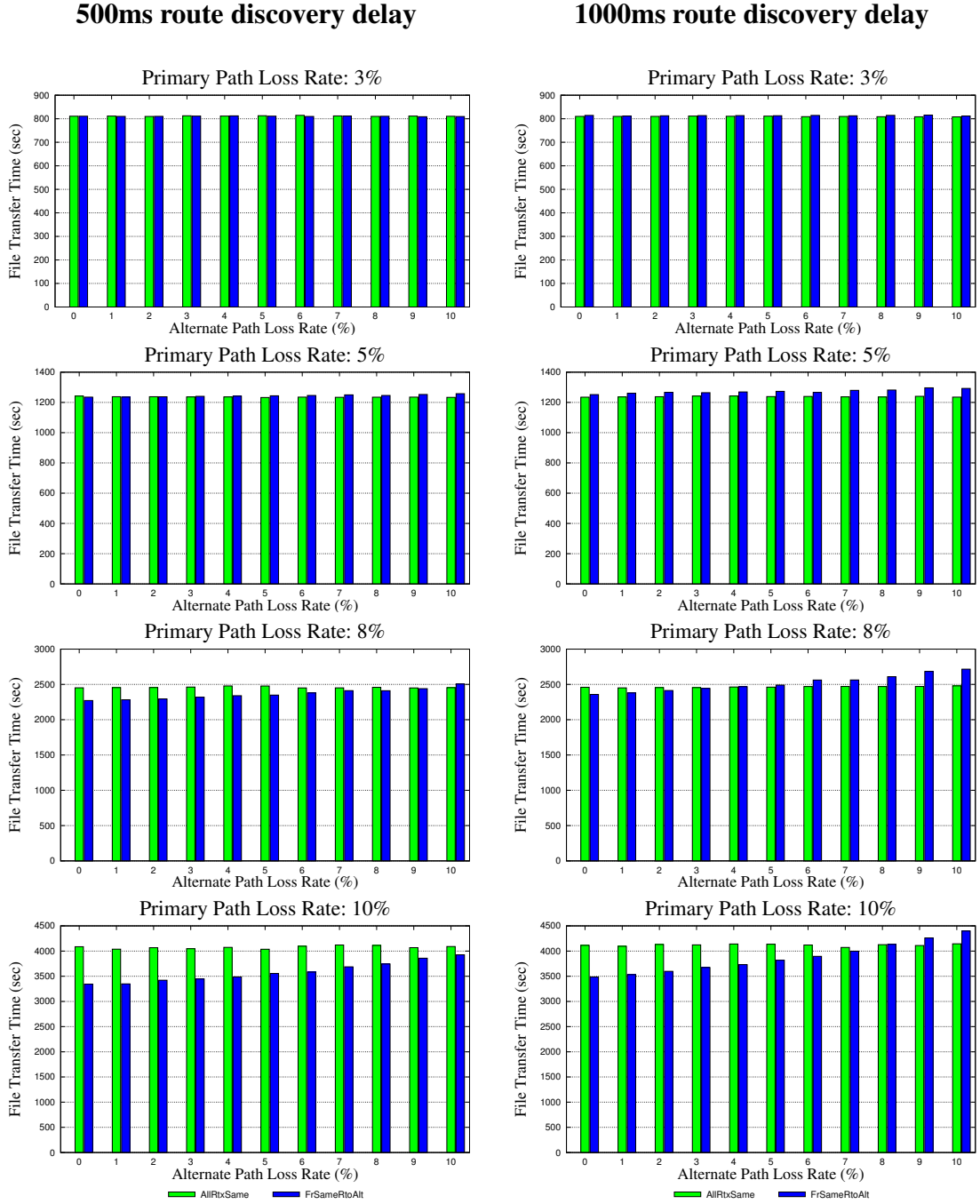
Figure 4.7: AllRtxSame and FrSameRtoAlt at {3, 5, 8, 10}% primary path loss, 90ms primary path RTT, 90ms alternate path RTT, 3200ms route cache lifetime, and {500, 1000}ms route discovery delay
