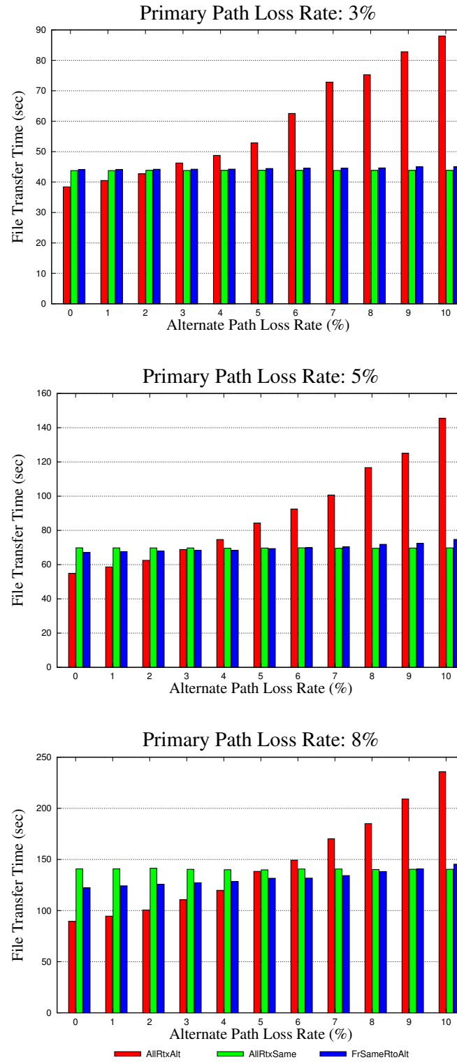
Figure 2.5: AllRtxAlt, AllRtxSame, and FrSameRtoAlt at {3, 5, 8}% primary path loss
