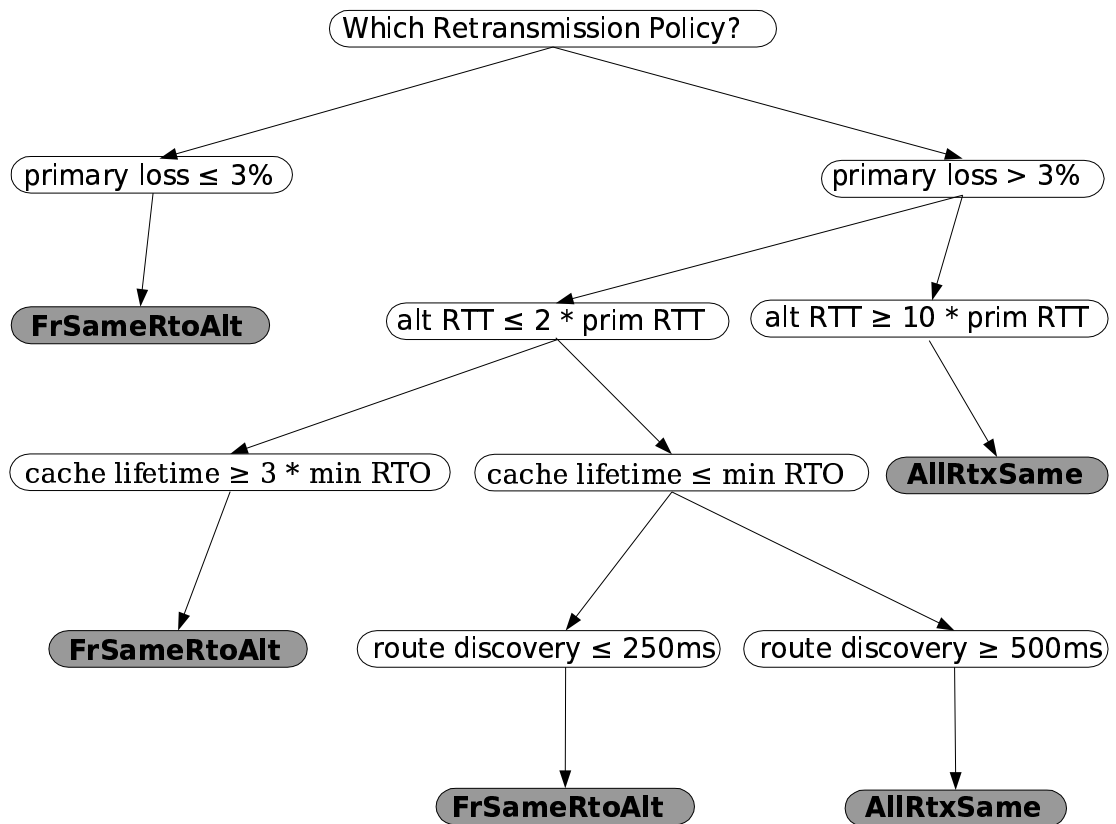
Figure 4.8: Retransmission policy suggestions
