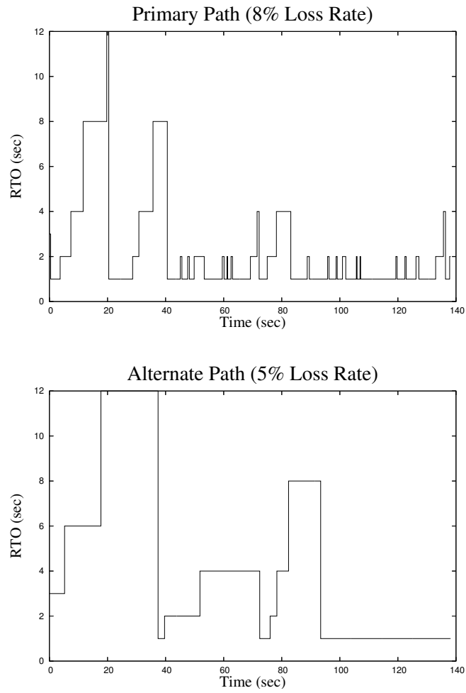
Figure 2.3: Example RTO dynamics with 8% primary path loss and 5% alternate path loss
