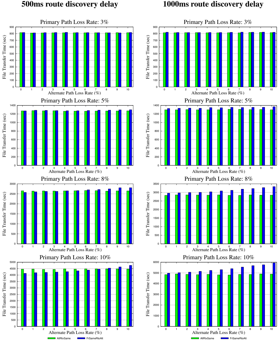
Figure 4.6: AllRtxSame and FrSameRtoAlt at {3, 5, 8, 10}% primary path loss, 90ms primary path RTT, 90ms alternate path RTT, 500ms route cache lifetime, and {500, 1000}ms route discovery delay
