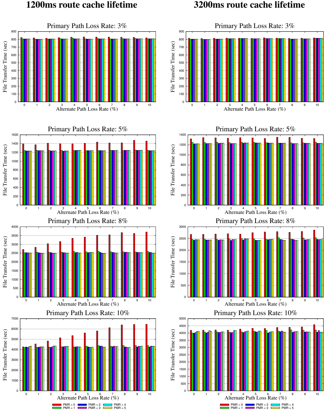
Figure 4.10: PMR settings with \{3, 5, 8, 10\}\% primary path loss, 90ms primary path RTT, 1040ms alternate path RTT, \{1200, 3200\} ms route cache lifetime, and 1000ms route discovery delay
