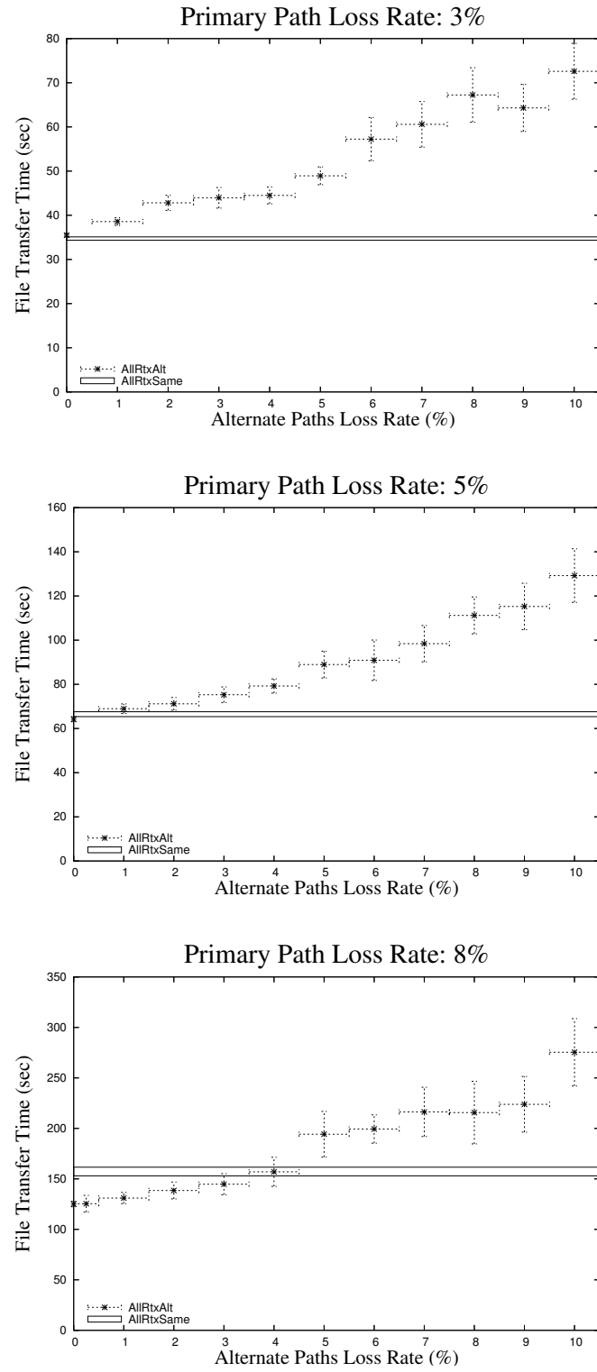
Figure 2.2: AllRtxAlt vs AllRtxSame at {3, 5, 8}% primary path loss
