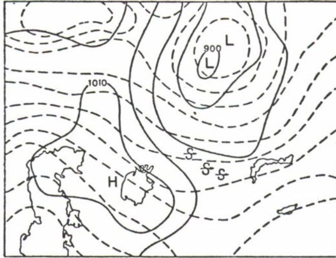
Figure 5. Dust storms in a high cyclone at Bet Pak Dala, Dzhetykonur, and Karsakpay stations, 1500 hours, 4 August 1957.
