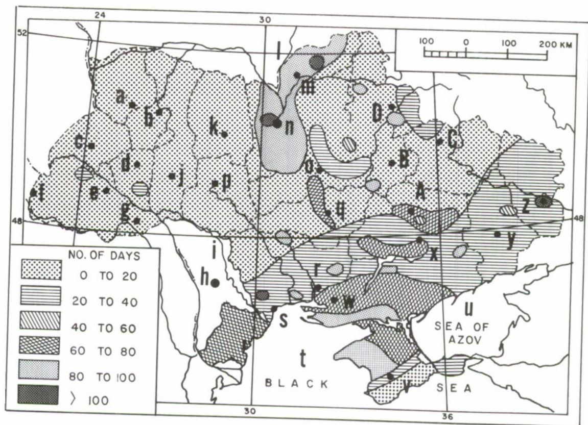
Figure 1. Number of days with dust storms in the Ukraine (for 20 years).
