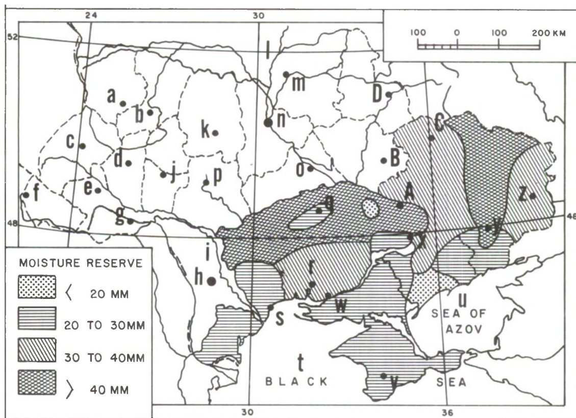
Figure 7. Moisture reserves in the plowed surface layer of soil in the spring of 1960.
