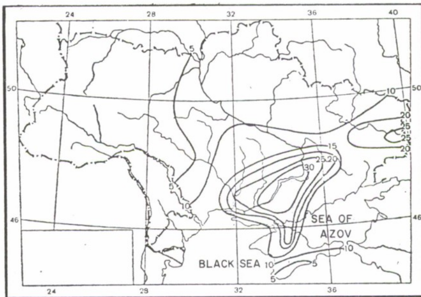
Figure 2. Maximum number of days with dust storms.
