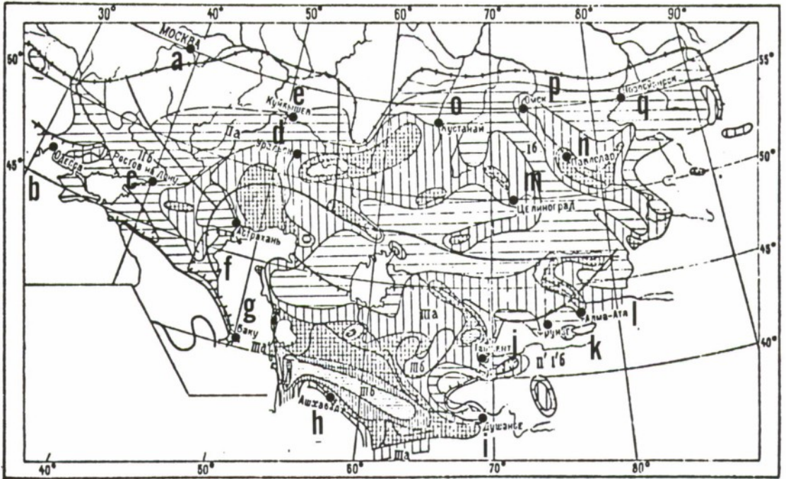
Figure 1. Number of days with dust storms.
