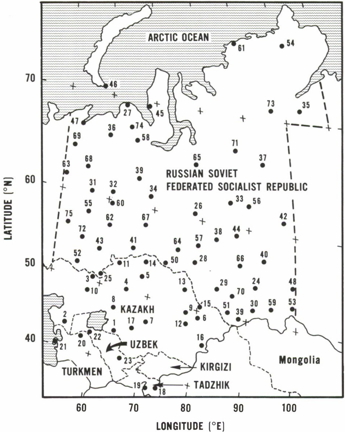
Figure 4. Station coverage for Soviet Central Asia - Kazakh, Tadzhik, Turkmen, Uzbek, and Russian Soviet Federated Socialist Republic. (See Table 2 for station summaries and data location.)
