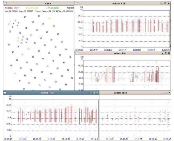
Figure 6: Range monitor display with hard limited spectrograms.
