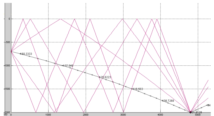
Figure 3. RayTrace for animal at 700 meters and hydrophone at a range of 4800 meters with the AUTECH 29 September 2005 SVP
