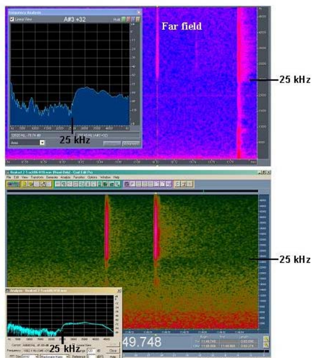
Figure 1. WHOI DTAG M. densirostris call spectra (top). Spectra of calls recorded at AUTC (bottom).
