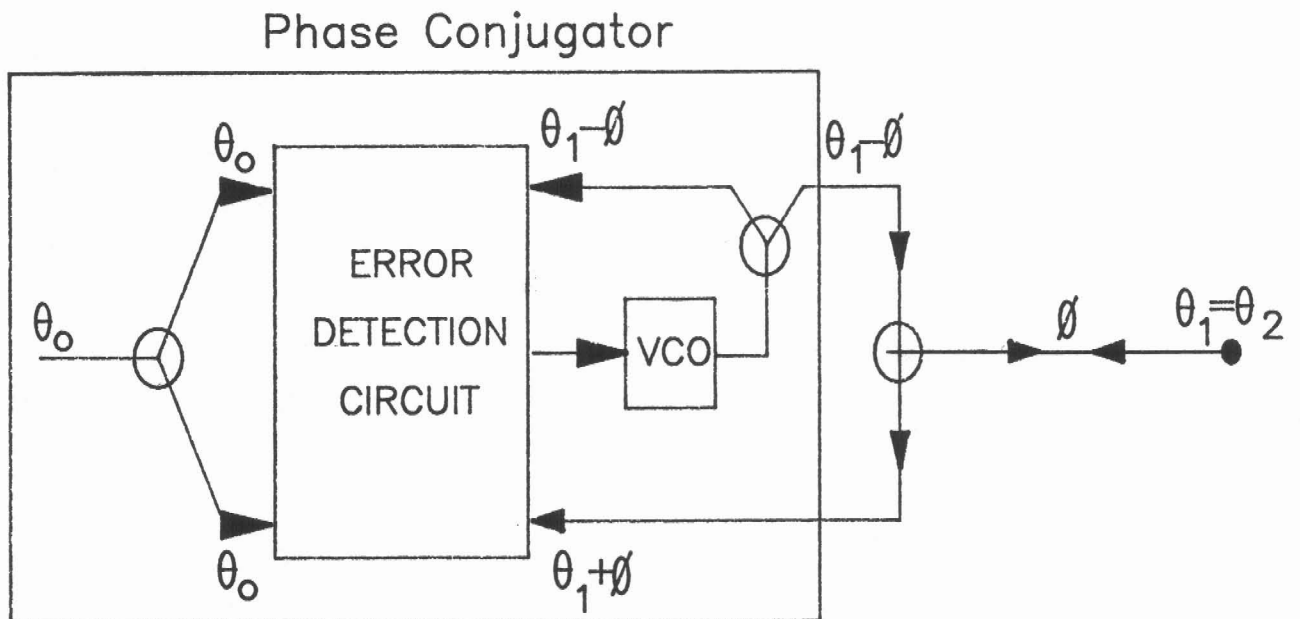
FIGURE 2. PHASE CONJUGATOR
