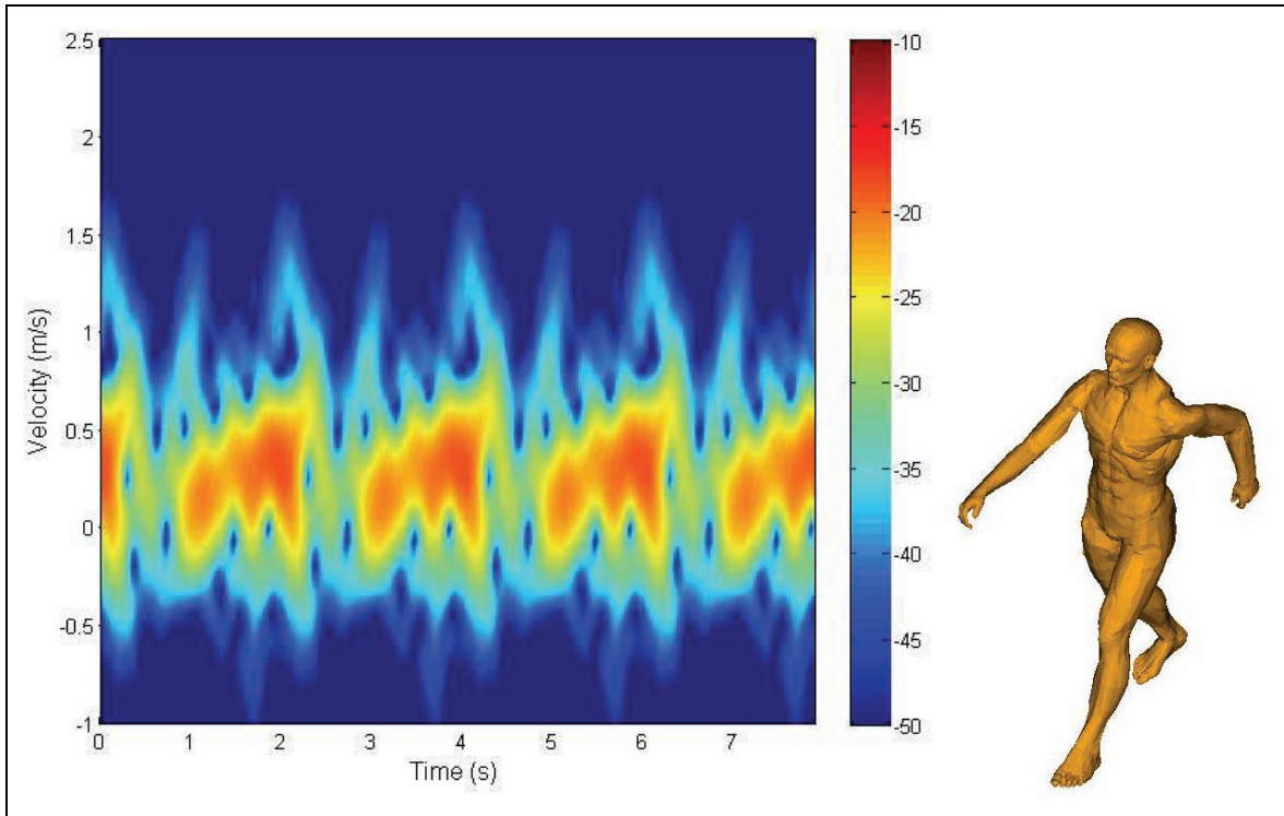
Figure 14. Spectrogram of the full human body in walking motion at 1 GHz, for a 60° azimuth incidence angle.
