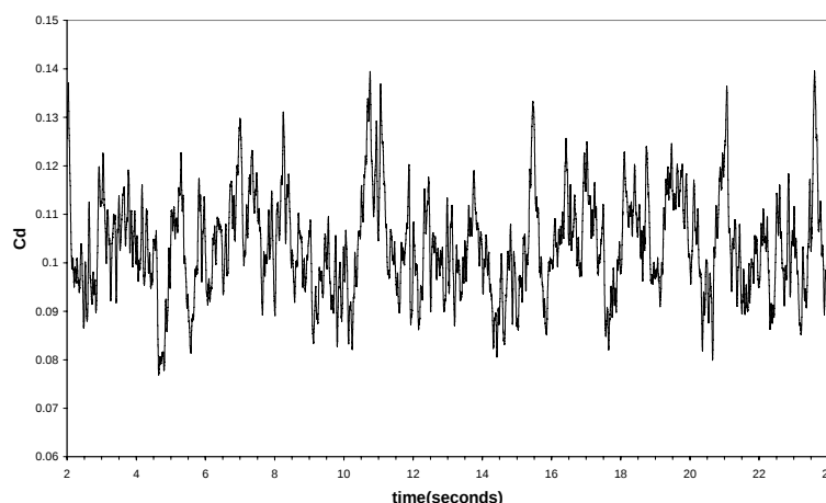
Figure 10: Drag coefficient versus time at Re = 1.0 \times 10^6
