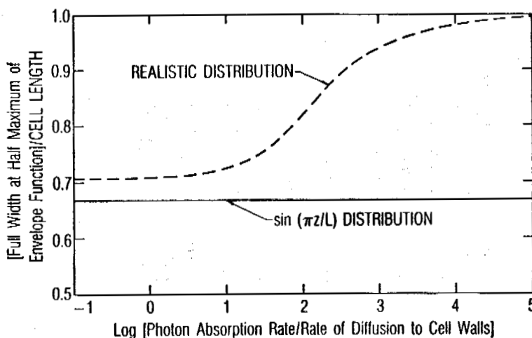
Figure 2: The full width at half maximum of the envelope function normalized to the resonance cell length as a function of the relative photon absorption rate. The true spatial distribution is always wider than what the first order diffusion mode would predict. However, when R/\gamma_{\text{diff}} \gtrsim 100 , there is a significant broadening of the spatial distribution of hyperfine polarization such that analysis based on a first order diffusion mode approximation is in error.
