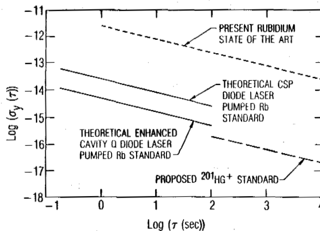
Figure 5: This figure is a comparison of diode laser pumped clocked performance with presently available rubidium standards and the proposed ^{201}\text{Hg}^+ standard. It should be noted, however, that while the projected stabilities of the diode laser pumped gas cell clock and mercury ion standard are similar, the mercury ion standard as presently envisaged has the potential to be a primary standard.
