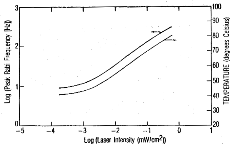
Figure 3: Using the non-empirical model of the gas cell atomic frequency standard, modified by the more appropriate envelope function discussed in the text, this figure shows the microwave Rabi frequencies and resonance cell temperatures that minimize the clock signals' shot noise Allan variance as a function of incident laser intensity.
