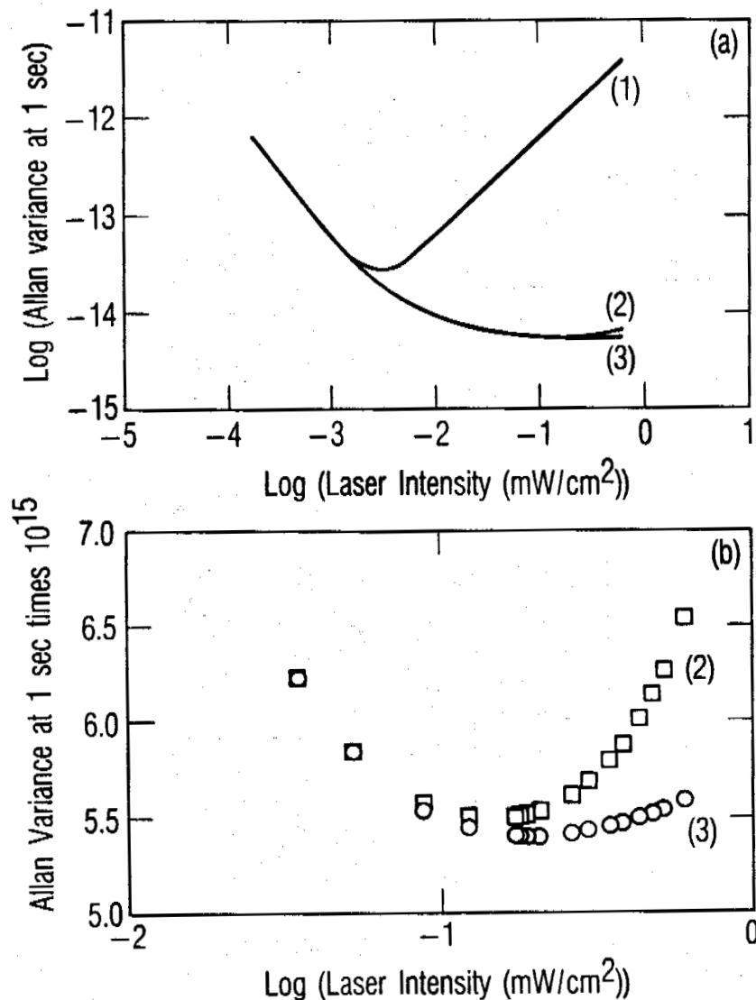
Figure 4: a) Curves 1, 2 and 3 illustrate the Allan variance at 1 second for a diode laser pumped Rb frequency standard with conditions (resonance cell temperature and microwave Rabi frequency) chosen in such a way that the clock signal's shot noise contribution is a minimum. Curve 1 assumes clock signal shot noise, diode laser quantum noise and diode laser frequency locking noise all contribute to the atomic clock's stability. Curve 2 assumes that only clock signal shot noise and diode laser frequency locking noise are important. Curve 3 shows the atomic clock's stability if only clock signal shot noise is present. Figure (b) is a magnification of Figure (a) in the region between 0.01 and 1 mW/cm 2 .
