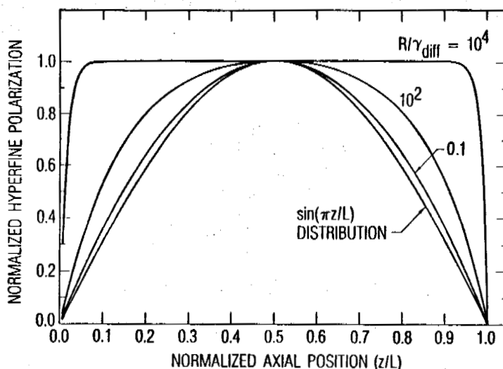
Figure 1: The envelope function f(z) describing the spatial distribution of hyperfine polarization \langle \vec{I} \cdot \vec{S} \rangle as a function of axial position within the resonance cell. The calculations assume that there is no collisional relaxation ( \gamma_1 = 0 ). Several curves are shown corresponding to relative values of the photon absorption rate R (i.e., R/\gamma_{\text{diff}} where \gamma_{\text{diff}} is a diffusional relaxation rate). These curves are to be compared with the first order axial diffusion mode \sin(\pi z/L) .
